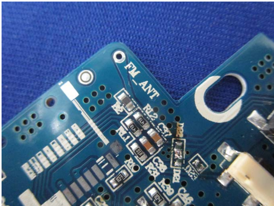
EUT –FM Antenna View
