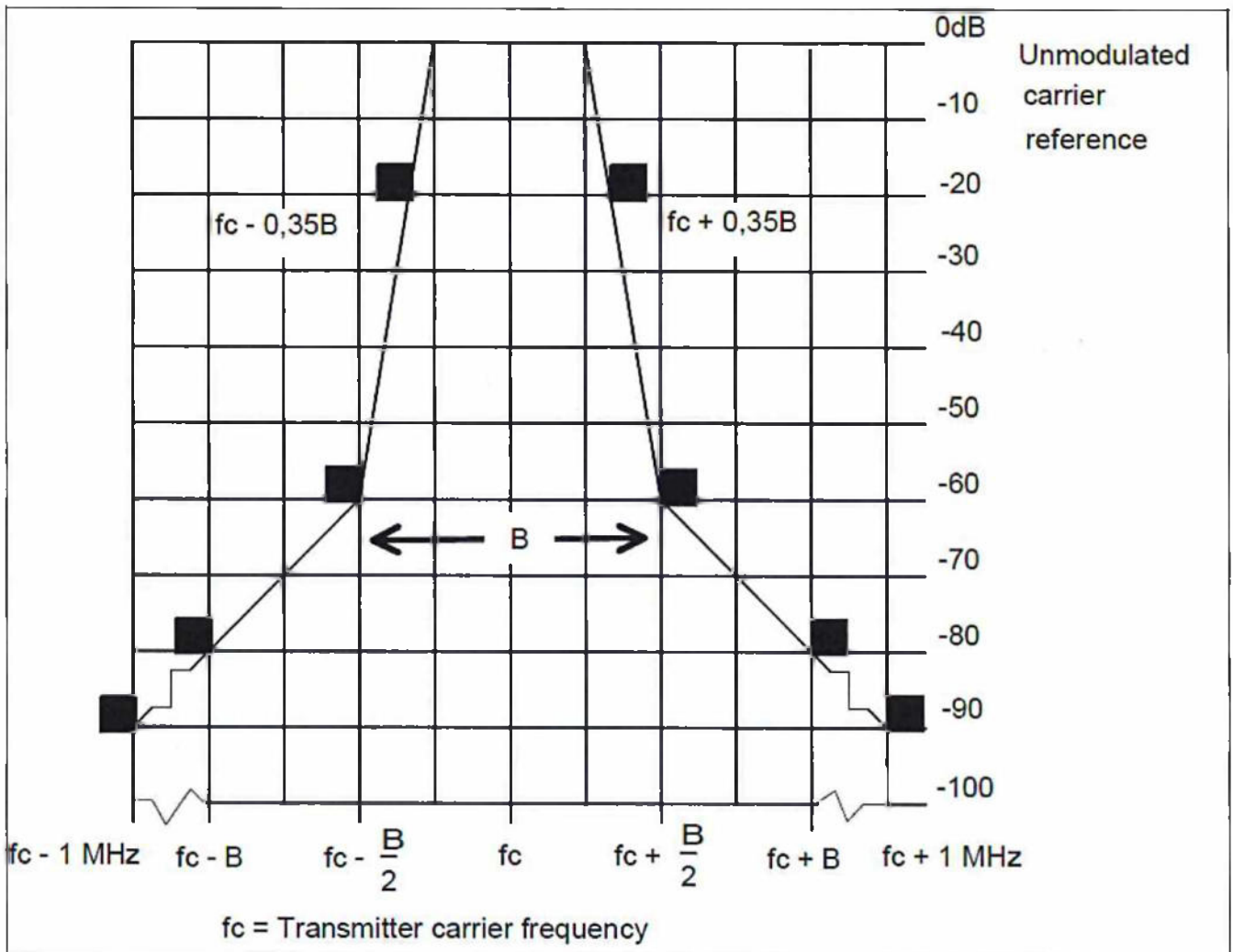
Figure 3 shows the spectrum mask for all analogue systems in the band. The -90 dBc point shall be \pm 1 \text{ MHz} from f_c measured with an average detector. To comply, a measured value shall fall below the mask limit as shown in figure 3.
