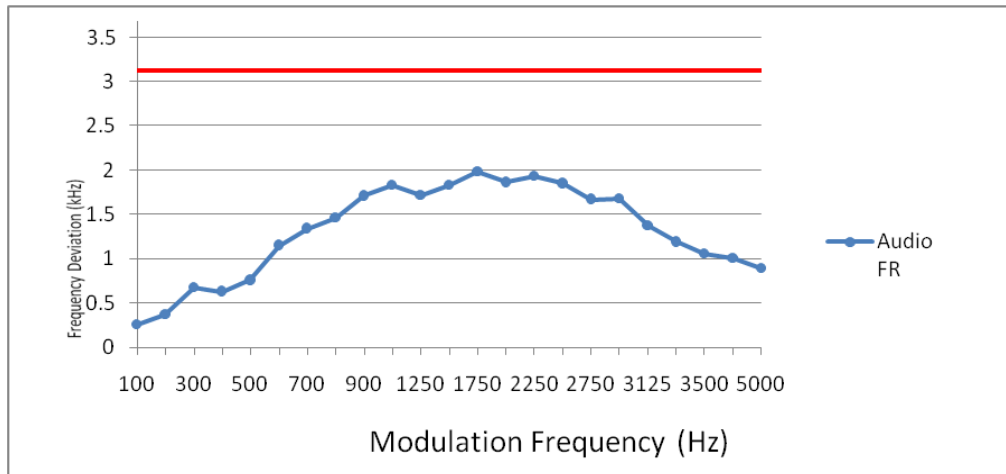
Audio Frequency Response
