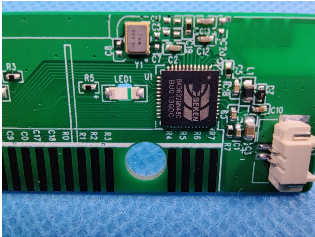
The series model is NS-PK3KCB24-C OPEN VIEW OF EUT (FIGURE 1)
