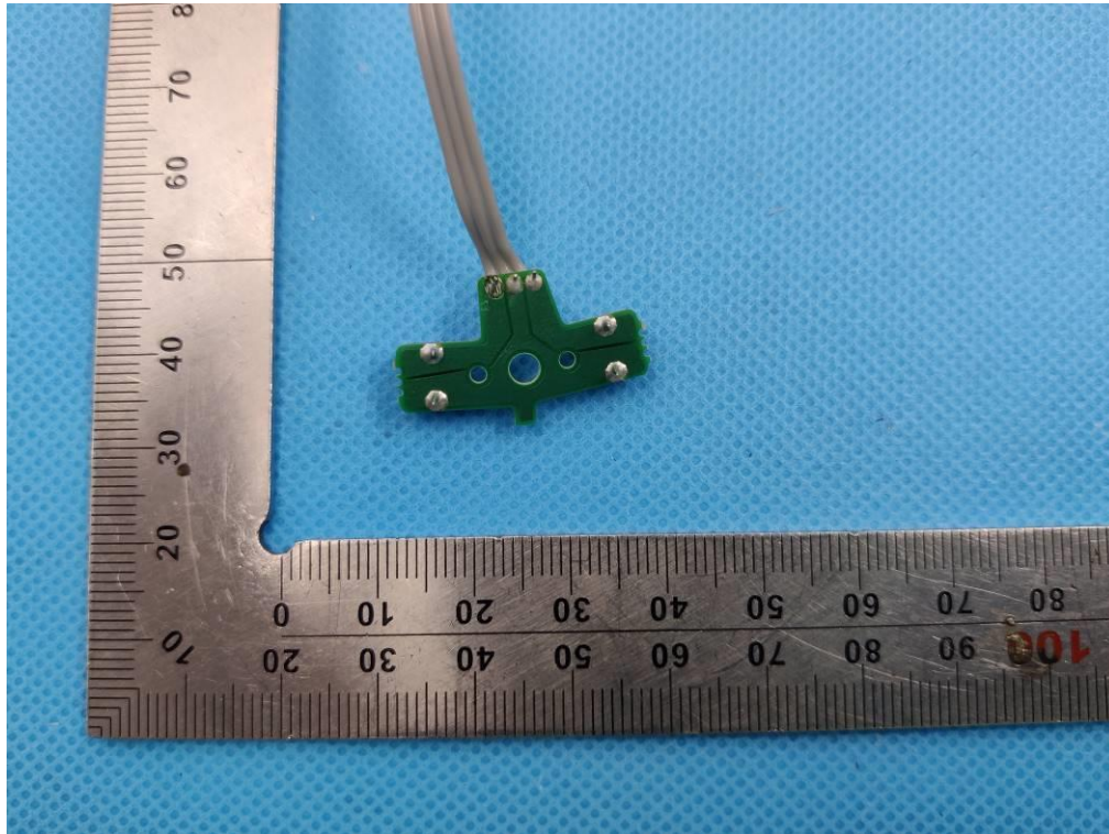
The series model is NS-PM4EK6B24-C OPEN VIEW OF EUT (FIGURE 1)
