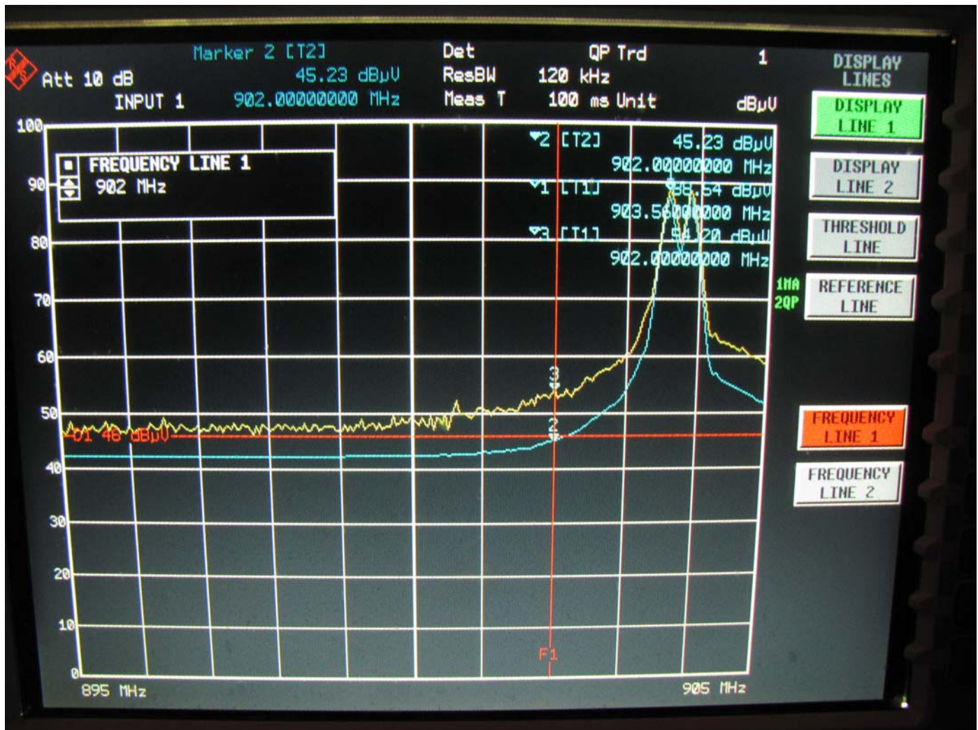
Band Edge for Low Channel – Horizontal Polarization – Y-Axis (Worst Case)
