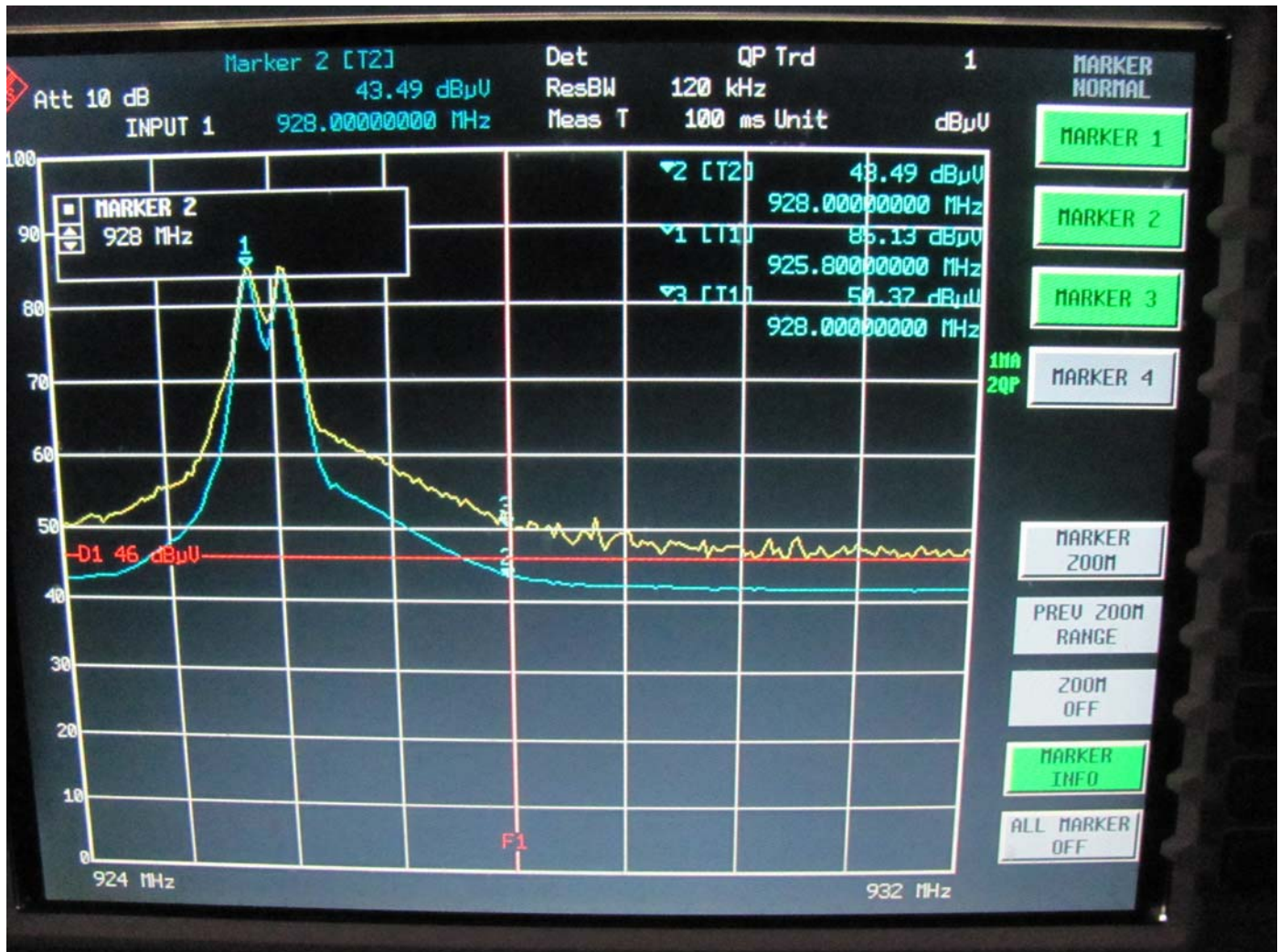
Band Edge for High Channel – Horizontal Polarization – Y-Axis (Worst Case)
