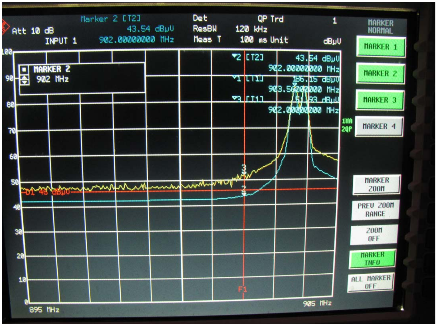
Band Edge for Low Channel – Vertical Polarization – Z-Axis (Worst Case)
