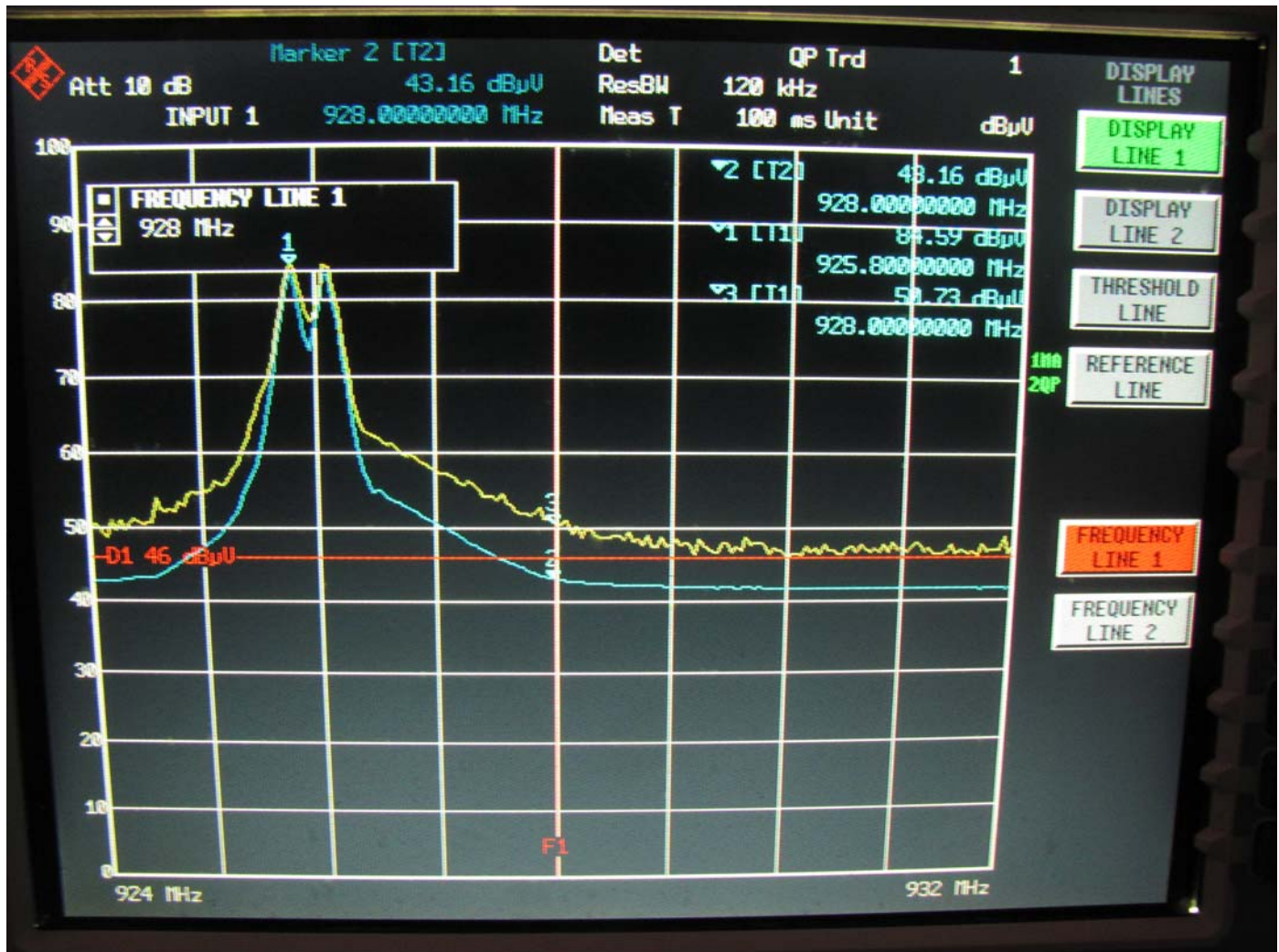
Band Edge for High Channel – Vertical Polarization – Z-Axis (Worst Case)
