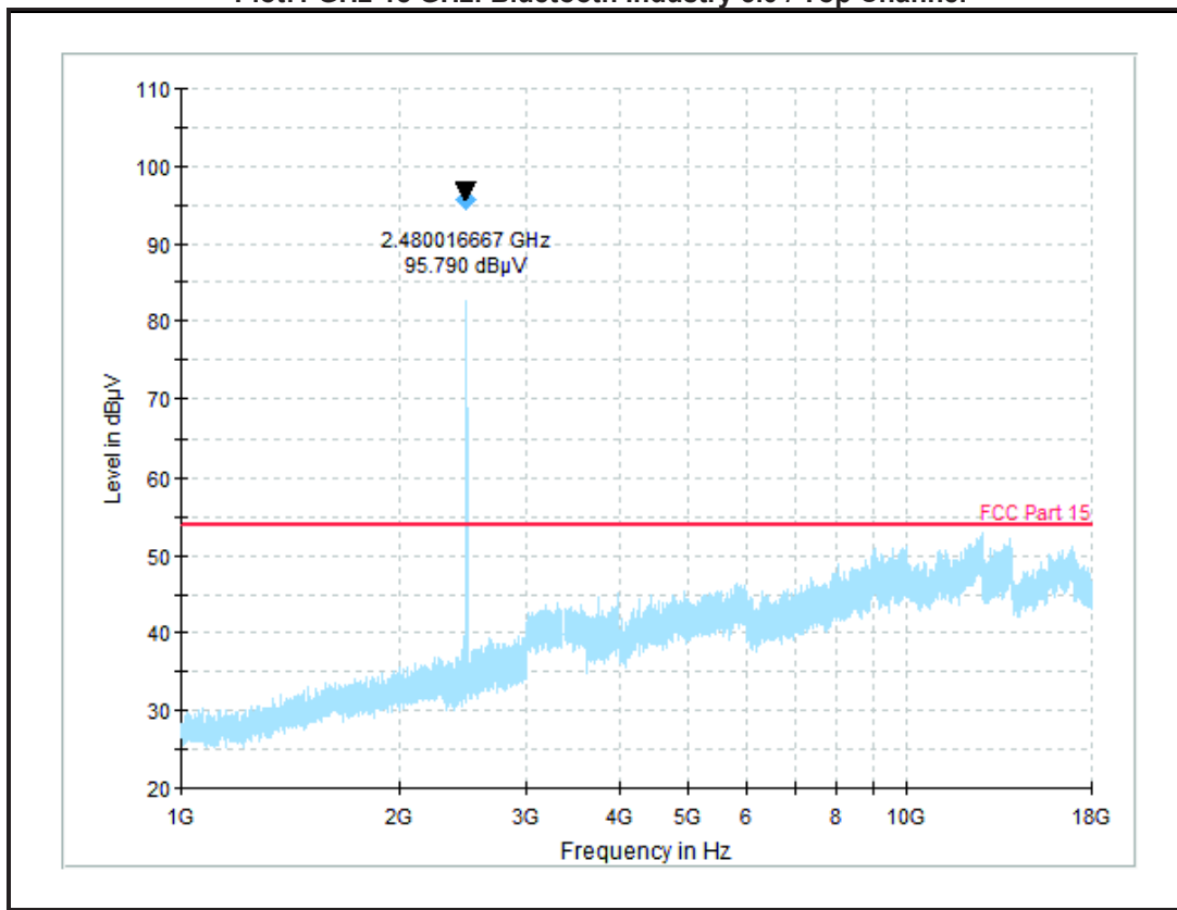
Plot: 1 GHz-18 GHz: Bluetooth Industry 5.0 / Top Channel
