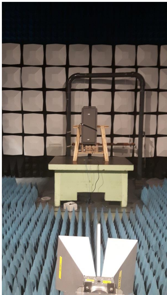
Test set up radiated emission 1GHz – 18 GHz
