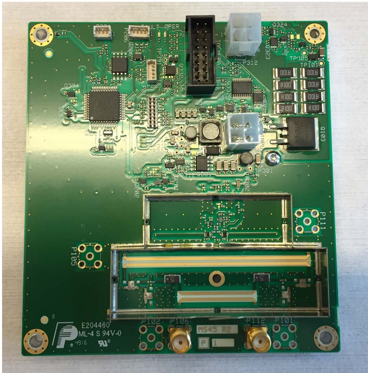
KS45.3 – Top no shields
