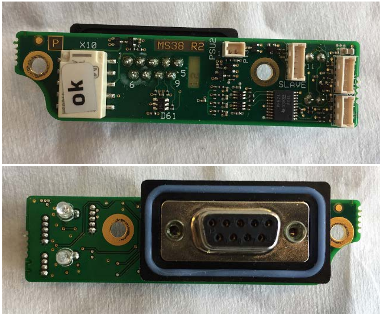
KS38.1 Top and Bottom
