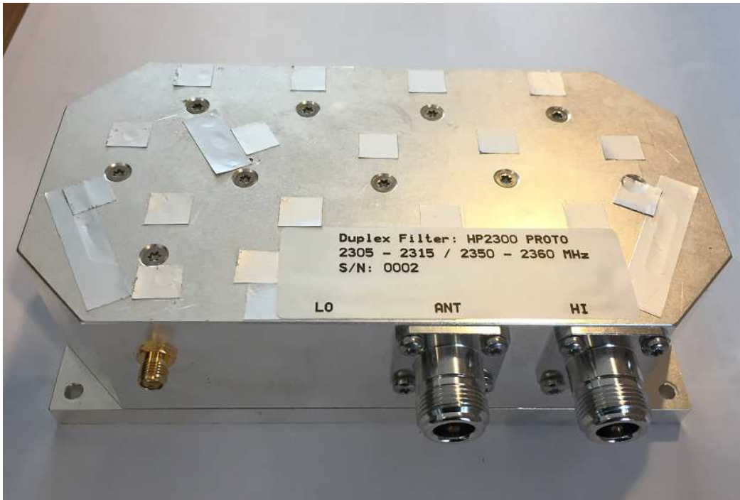
Duplex Filter side
