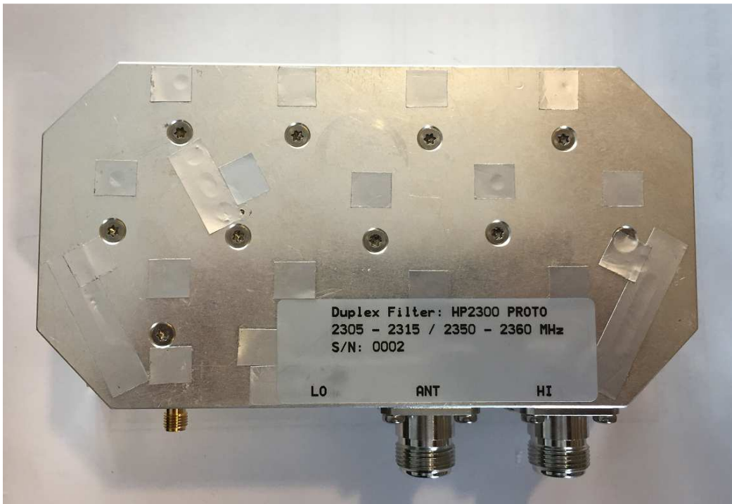
Duplex Filter top
