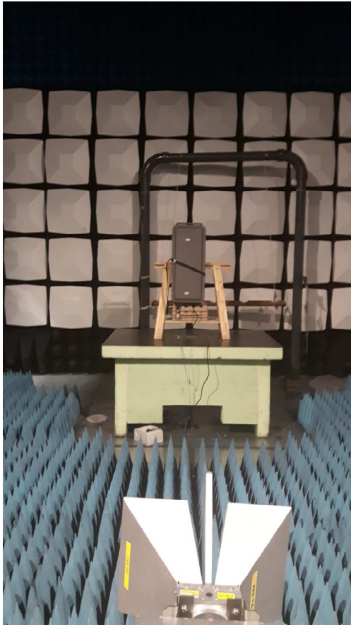
Test set up radiated emission 1GHz – 18 GHz
