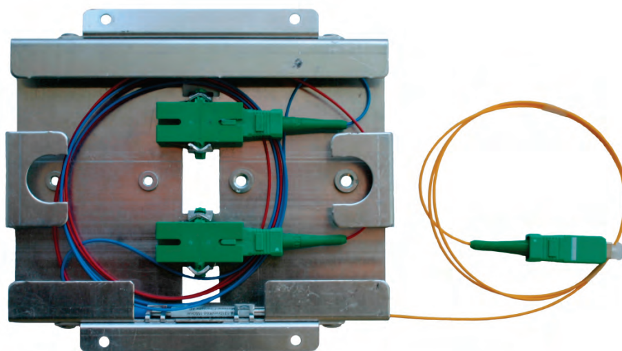
FOR Mux Assembly Bottom view
