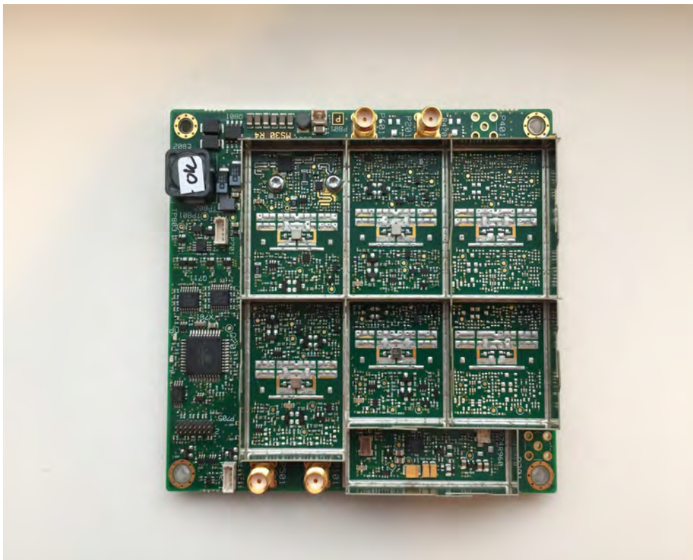
VGA 700 Board, Top view, without shields
