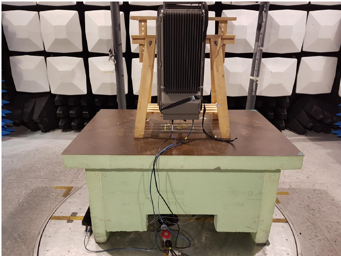
Test Set up radiated emission: EUT
