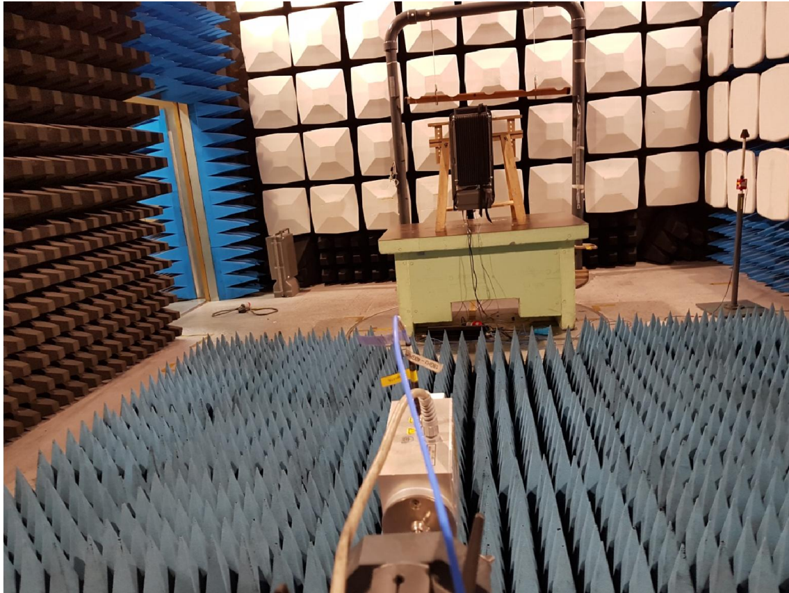
Test set up radiated emission 18 GHz – 26.5 GHz
