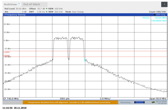
Figure 8.5-2: 738.5 and 743.5 MHz AGC + 3 dB Out-of-block DL
