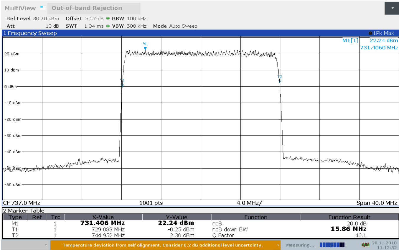
Figure 8.2-1: Passband Downlink
