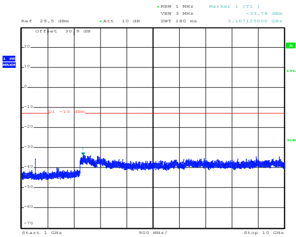
Figure 8.6-2: 1-10 GHz 728 MHz
