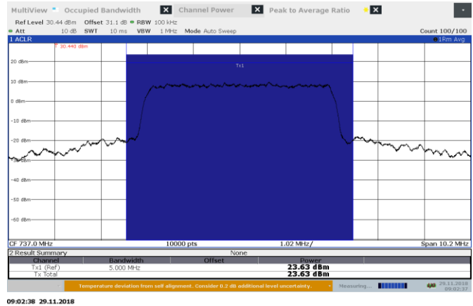
Figure 8.4-2: AGC -0.5 dB 737 MHz Output DL
