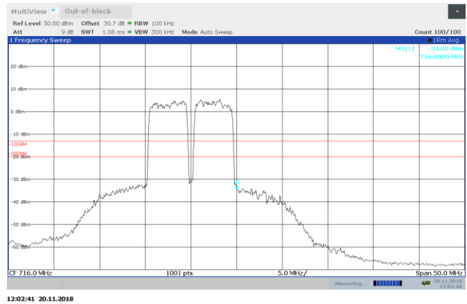
Figure 8.5-10: 708.5 and 713.5 MHz AGC + 3 dB Out-of-block UL
