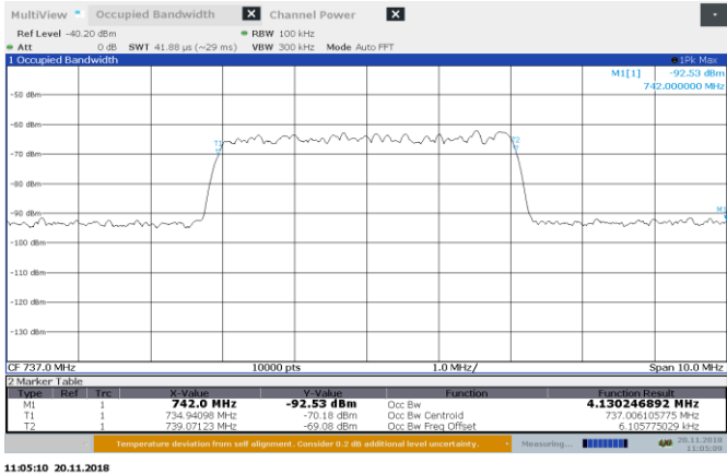
Figure 8.3-3: AGC +3 dB 737 MHz input 99% BW DL
