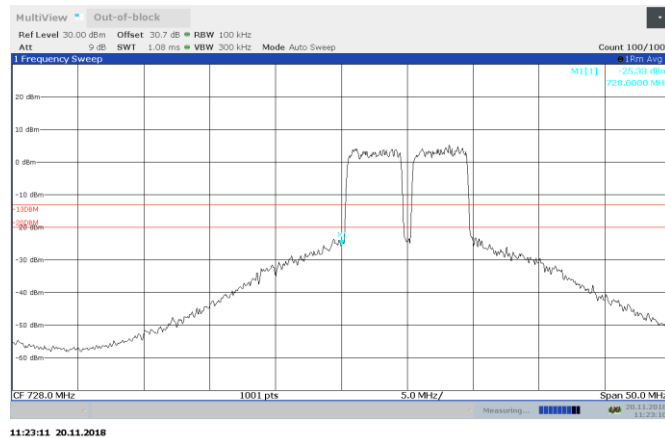
Figure 8.5-3: 730.5 and 735.5 MHz AGC - 0.5dB Out-of-block DL
