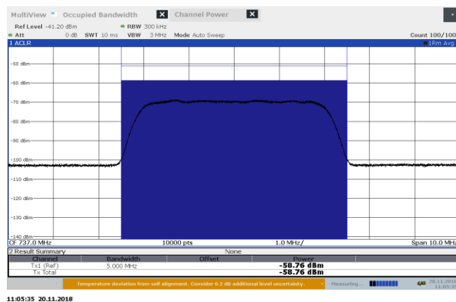
Figure 8.1-1: AWGN AGC +1 dB 737 MHz input DL
