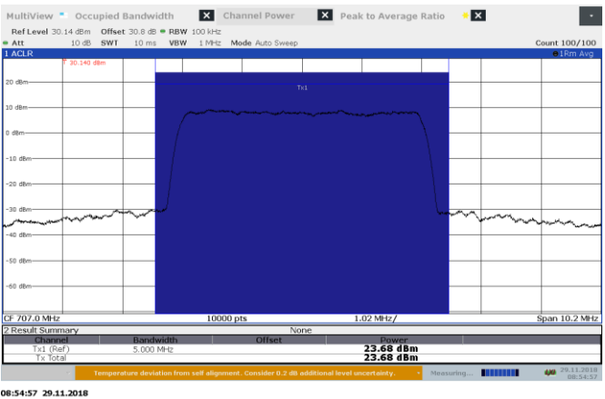
Figure 8.4-6: AGC -0.5 dB 707 MHz Output UL
