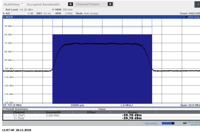
Figure 8.4-1: AGC -0.5 dB 737 MHz Input DL
