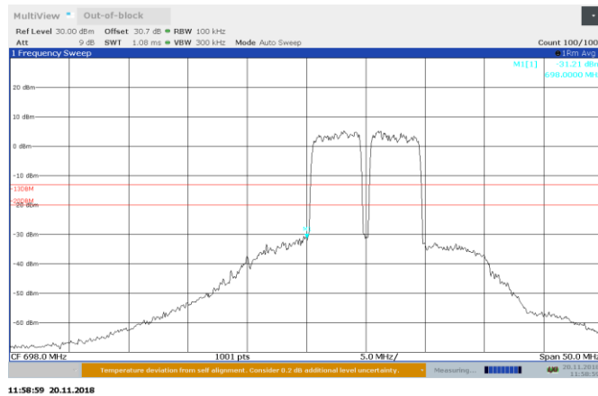
Figure 8.5-11: 700.5 and 705.5 MHz AGC - 0.5dB Out-of-block UL
