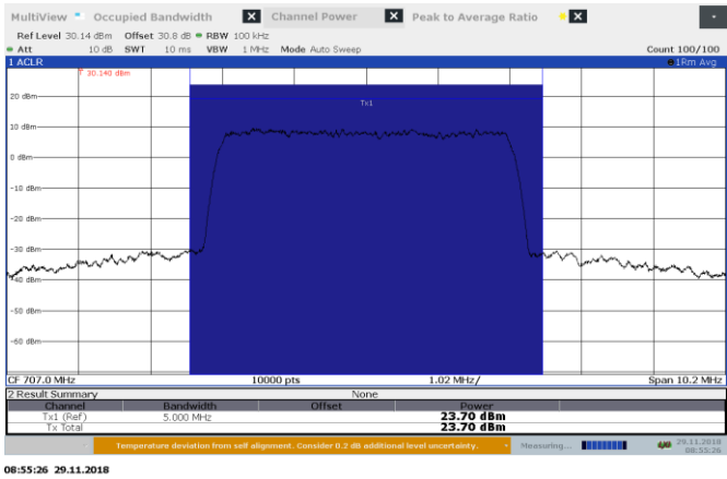
Figure 8.4-7: AGC +3 dB 707 MHz Output UL
