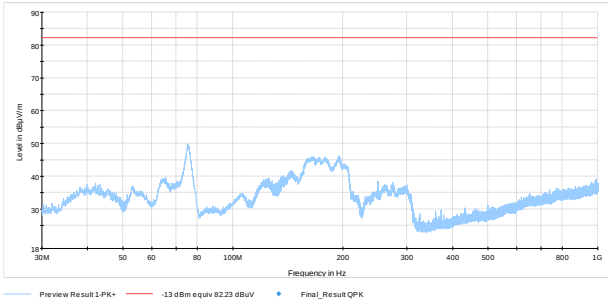
Figure 8.7-3: 30 MHz to 1 GHz DL
