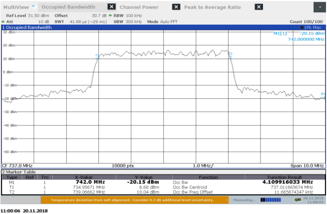
Figure 8.3-2: AGC-0.5 dB 737 MHz output 99% BW DL
