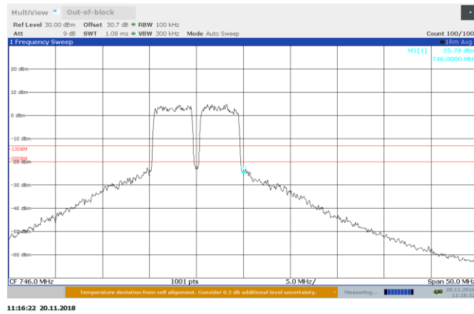
Figure 8.5-1: 738.5 and 743.5 MHz AGC - 0.5dB Out-of-block DL
