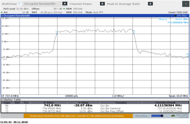
Figure 8.3-4: AGC +3 dB 737 MHz output 99% BW DL
