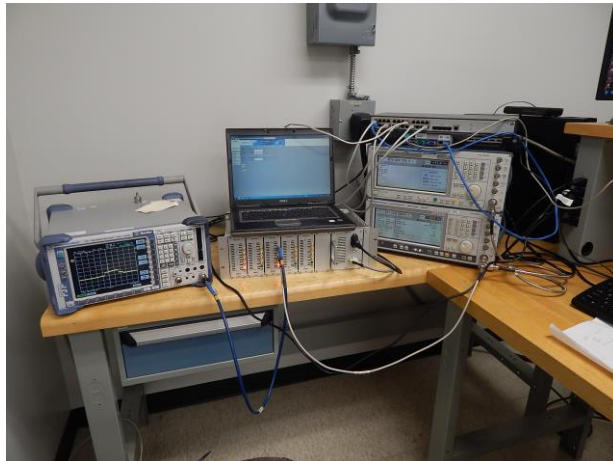
Figure 9.1-2: Conducted setup photo
