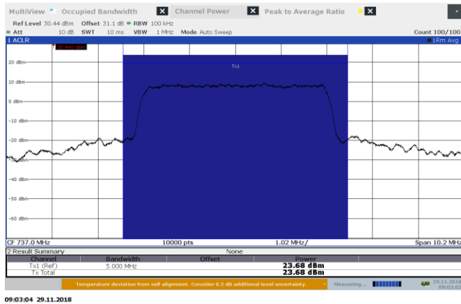
Figure 8.4-3: AGC +3 dB 737 MHz Output DL
