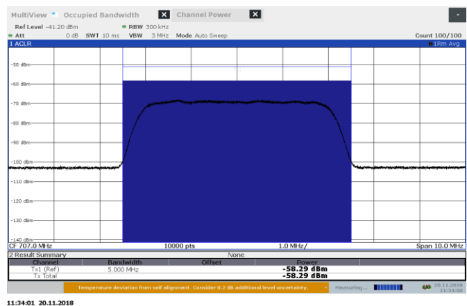
Figure 8.1-2: AGC +1 dB 707 MHz input UL
