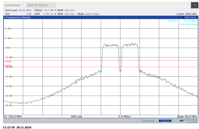
Figure 8.5-4: 730.5 and 735.5 MHz AGC + 3 dB Out-of-block DL
