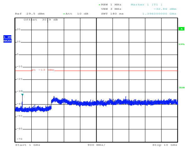
Figure 8.6-6: 1-10 GHz 746 MHz
