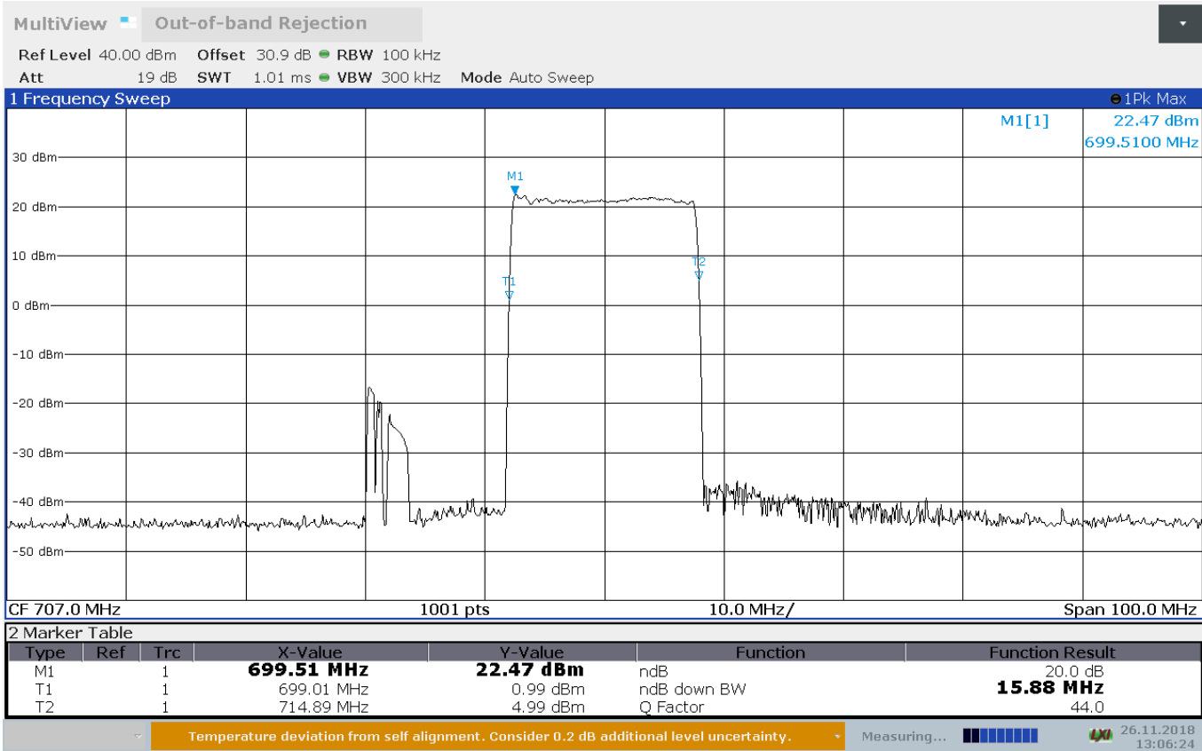
Figure 8.2-3: Passband Uplink 100MHz Span
