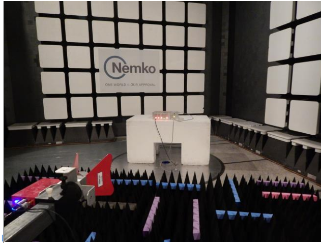
Figure 9.1-1: Radiated setup photo
