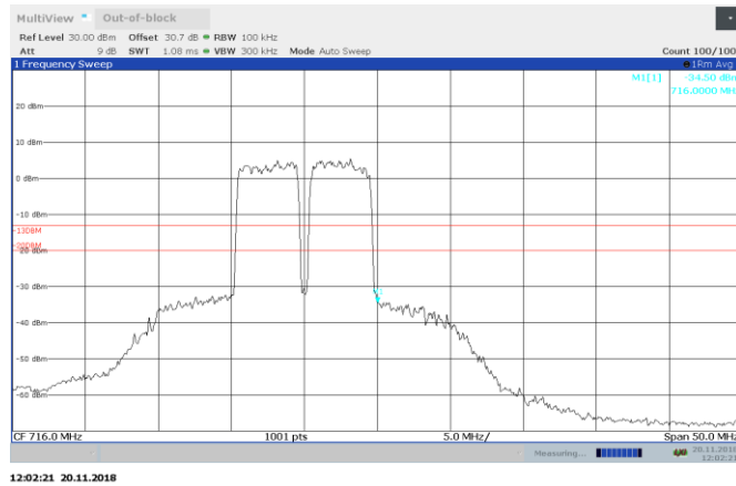
Figure 8.5-9: 708.5 and 713.5 MHz AGC - 0.5dB Out-of-block UL
