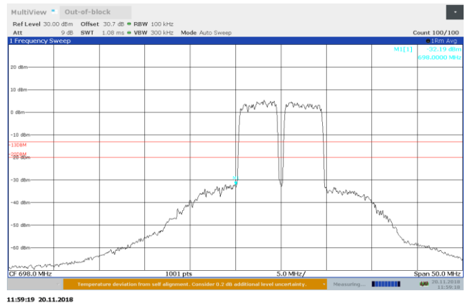
Figure 8.5-12: 700.5 and 705.5 MHz AGC + 3 dB Out-of-block UL
