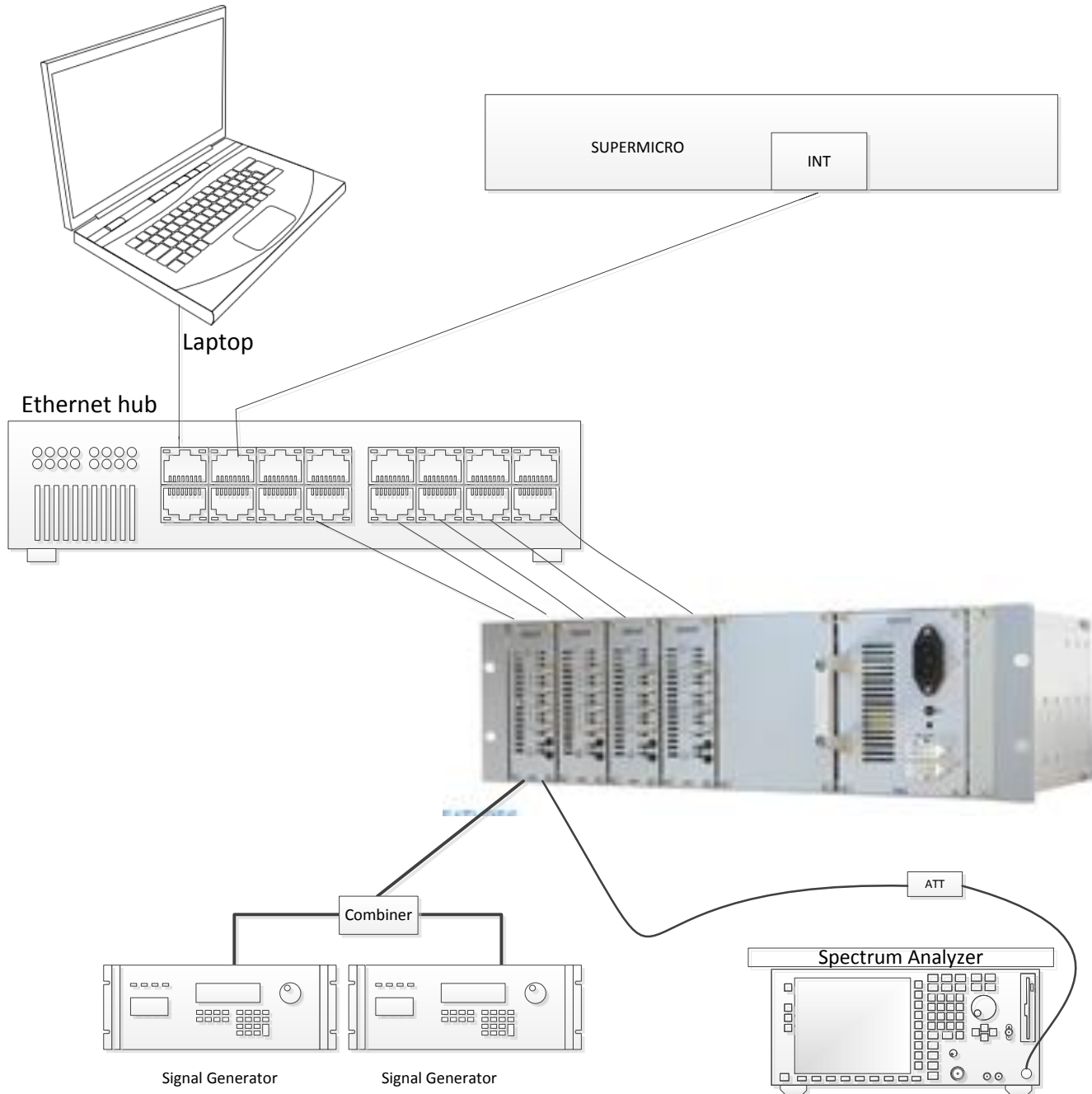
Figure 3.6-1: Setup diagram
