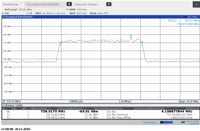
Figure 8.3-1: AGC-0.5 dB 737 MHz input 99% BW DL
