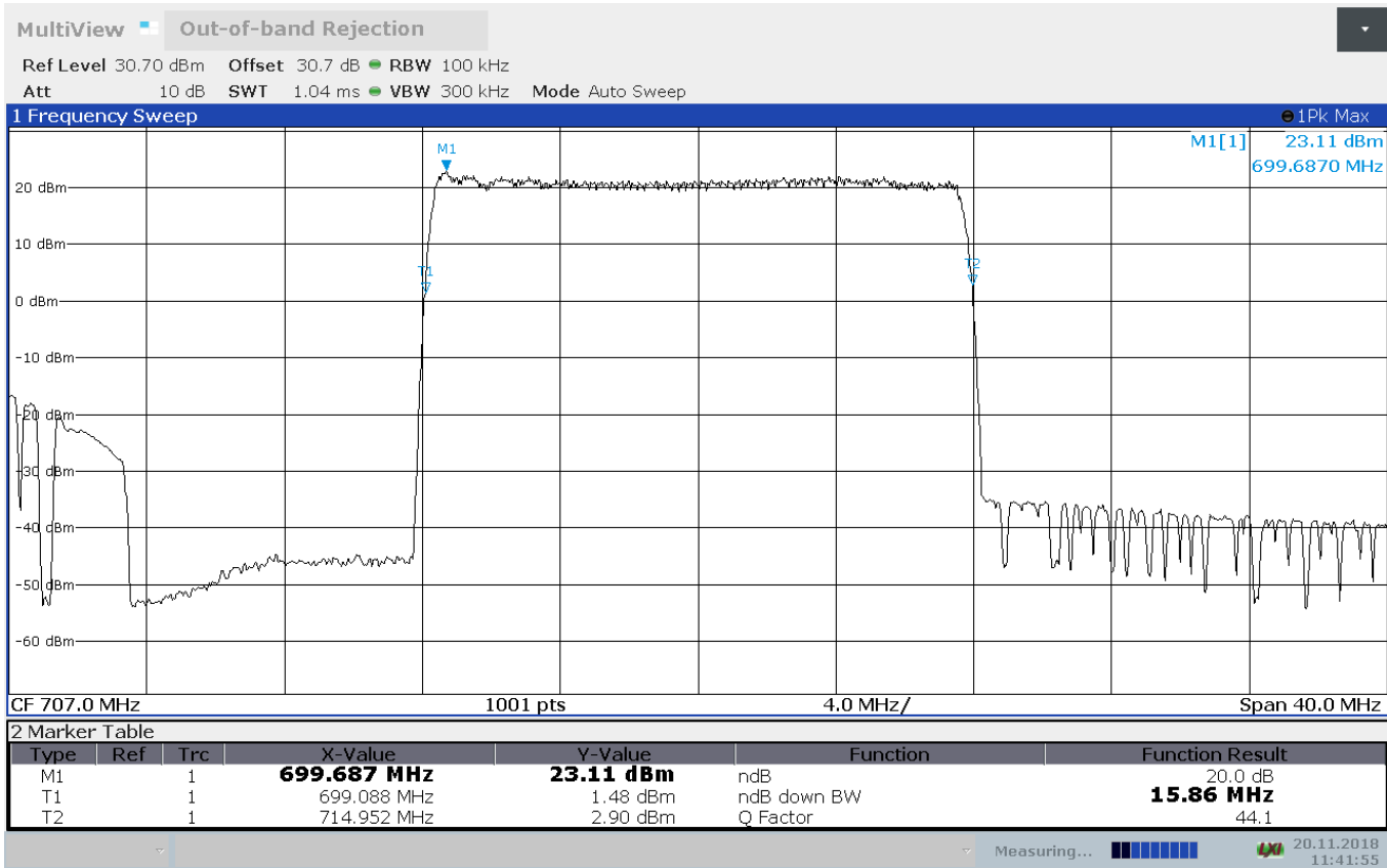
Figure 8.2-2: Passband Uplink
