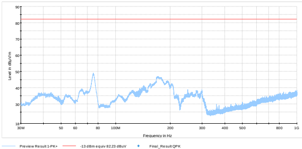
Figure 8.7-1: 30 MHz to 1 GHz UL
