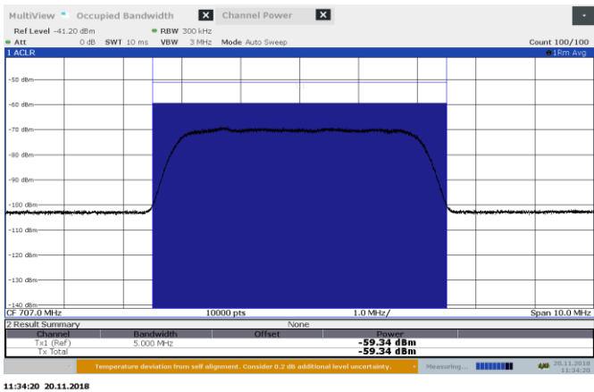
Figure 8.4-5: AGC -0.5 dB 707 MHz Input UL
