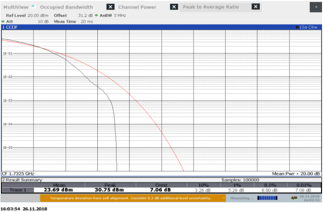
Figure 8.4-4: AWGN AGC—0.5 dB 1732.5 MHz PAPR UL
