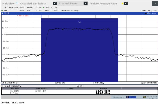
Figure 8.4-3: AWGN AGC +3dB 1732.5 MHz output UL
