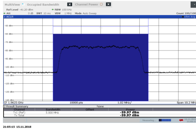
Figure 8.4-1: AWGN AGC—0.5 dB 1962.5 MHz Input DL
