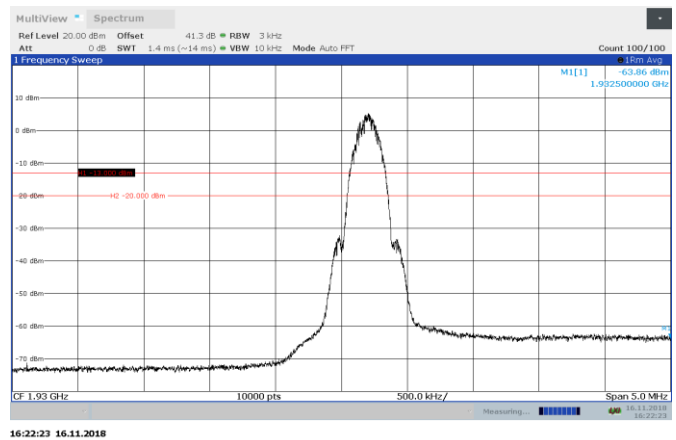
Figure 8.5-32: MSK 1930.2 MHz AGC + 3dB Out-of-block DL
