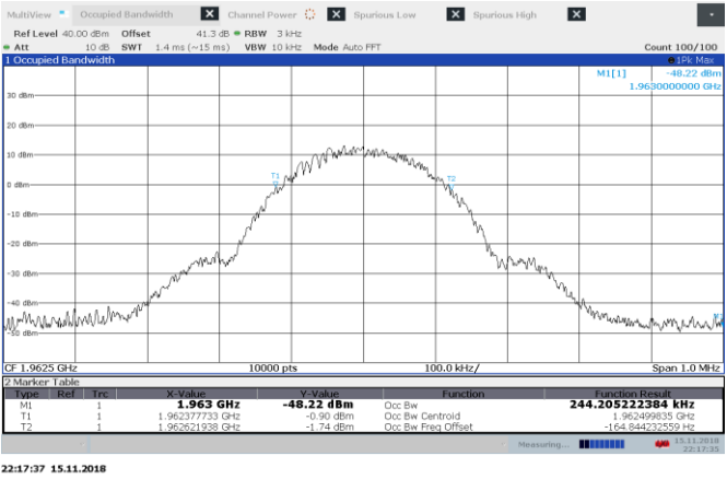
Figure 8.3-8: MSK AGC +3 dB 1962.5 MHz output 99% BW DL
