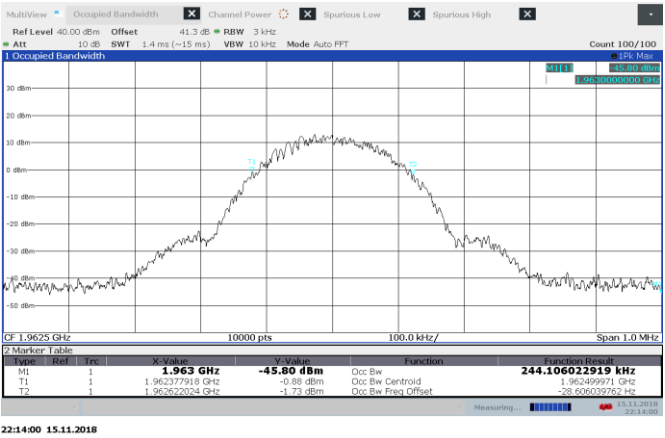
Figure 8.3-6: MSK AGC -0.5 dB 1962.5 MHz output 99% BW DL
