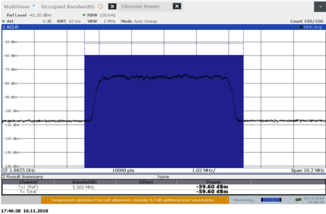
Figure 8.4-13: AWGN AGC—0.5 dB 1882.5 MHz Input UL
