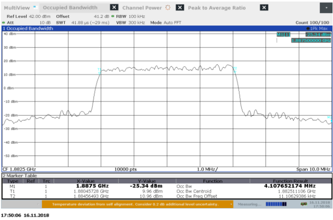
Figure 8.3-16: AWGN AGC +3 dB 1882.5 MHz output 99% BW UL
