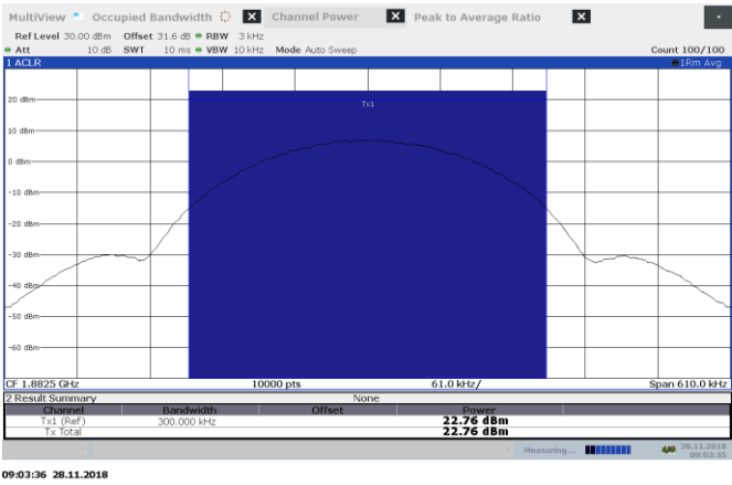
Figure 8.4-10: MSK AGC—0.5 dB 1882.5 MHz Output UL
