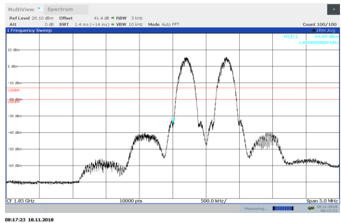
Figure 8.5-12: MSK 1850.2 and 1850.8 MHz AGC + 3dB Out-of-block UL
