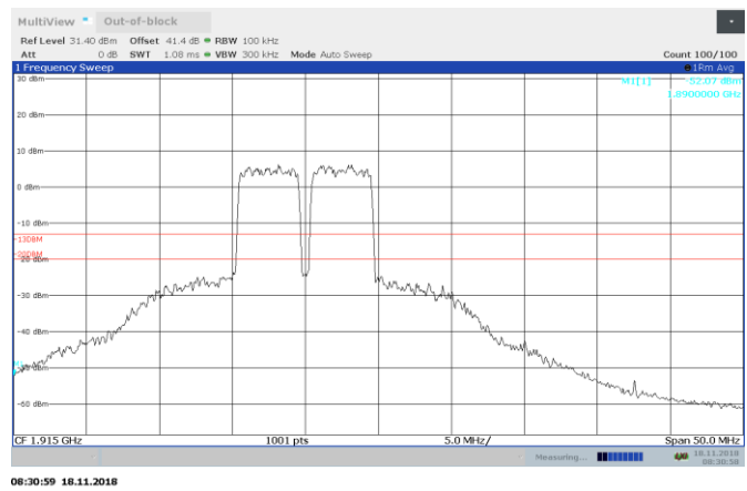
Figure 8.5-2: AWGN 1907.5 and 1912.5 MHz AGC + 3dB Out-of-block UL
