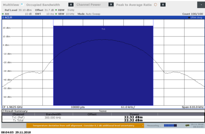
Figure 8.4-7: MSK AGC+ 3dB 1962.5 MHz Output DL
