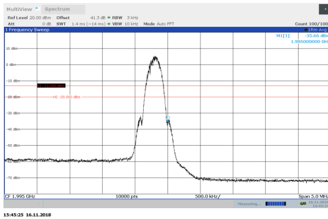
Figure 8.5-29: MSK 1994.8 MHz AGC - 0.5dB Out-of-block DL
