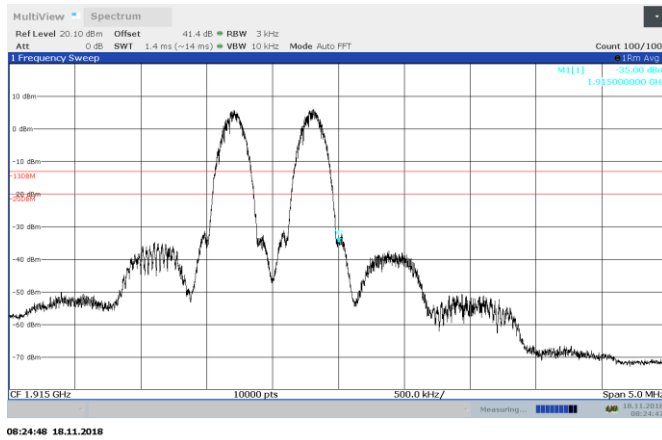
Figure 8.5-9: MSK 1914.2 and 1914.8 MHz AGC - 0.5dB Out-of-block UL
