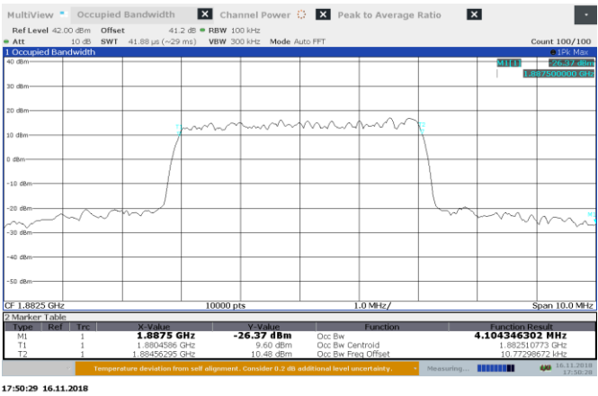
Figure 8.3-14: AWGN AGC -0.5 dB 1882.5 MHz output 99% BW UL
