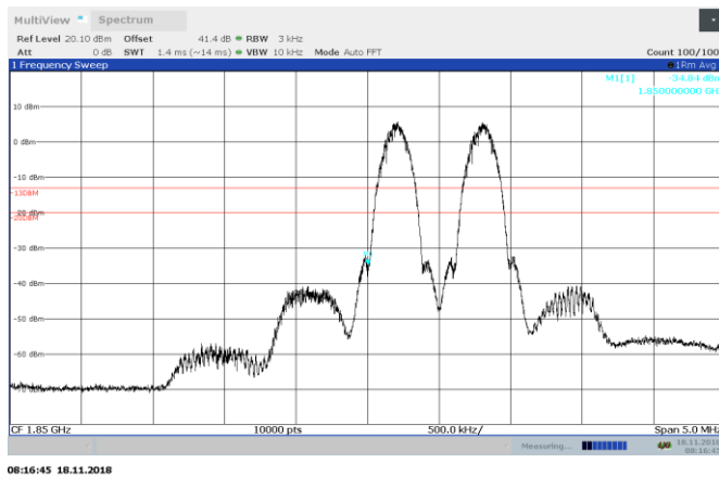
Figure 8.5-11: MSK 1850.2 and 1850.8 MHz AGC - 0.5dB Out-of-block UL
