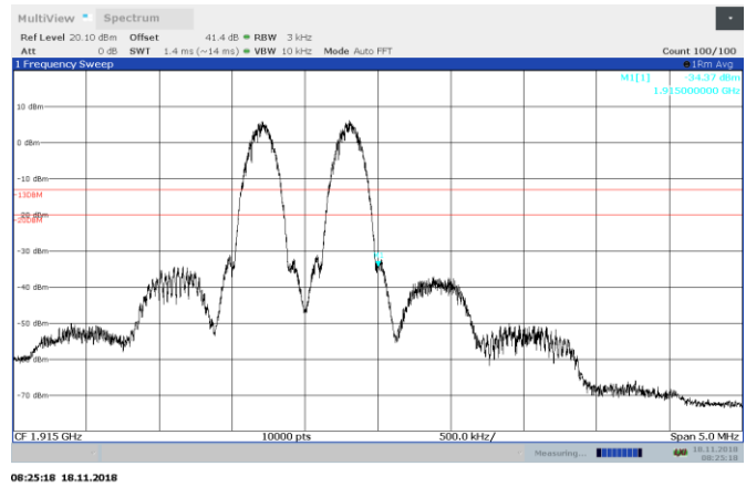
Figure 8.5-10: MSK 1914.2 and 1914.8 MHz AGC +3dB Out-of-block UL
