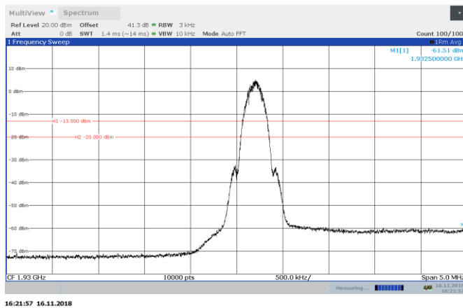
Figure 8.5-31: MSK 1930.2 MHz AGC - 0.5dB Out-of-block DL
