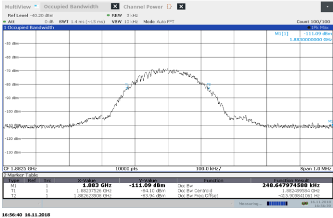
Figure 8.3-9: MSK AGC-0.5 dB 1882.5 MHz input 99% BW UL
