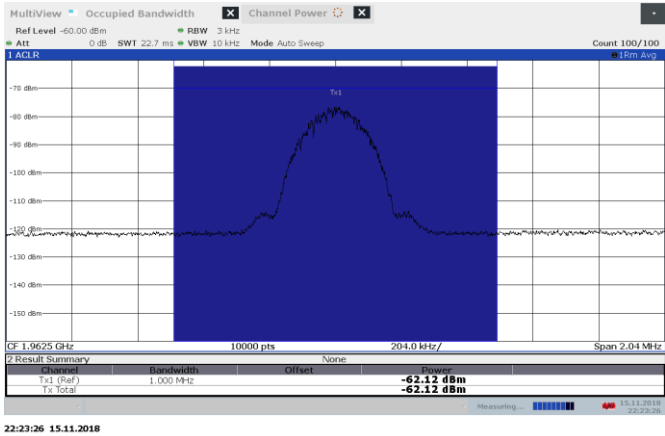
Figure 8.4-5: MSK AGC—0.5 dB 1962.5 MHz Input DL
