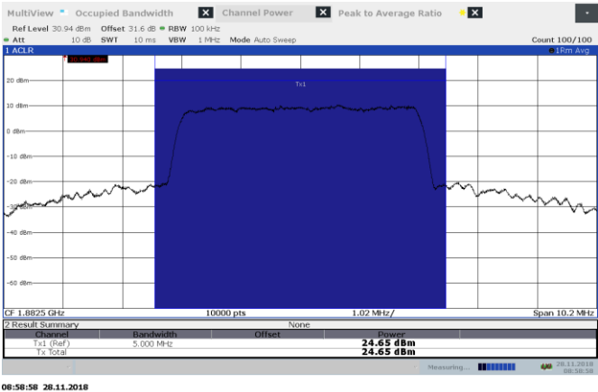
Figure 8.4-15: AWGN AGC+ 3dB 1882.5 MHz Output UL
