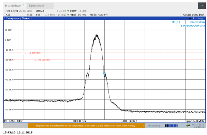
Figure 8.5-30: MSK 1994.8 MHz AGC + 3dB Out-of-block DL
