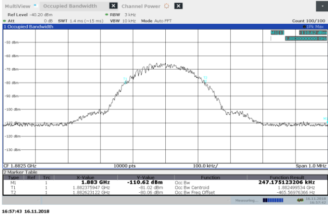
Figure 8.3-11: MSK AGC+3 dB 1882.5 MHz input 99% BW UL
