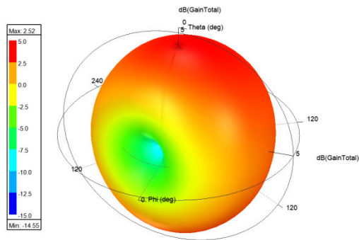
Antenna Gain 3D, 2.48-GHz
