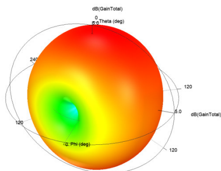
Antenna Gain 3D, 2.48-GHz
