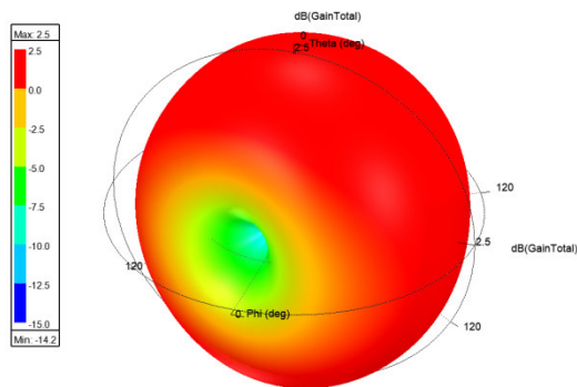
Antenna Gain 3D, 2.448GHz
