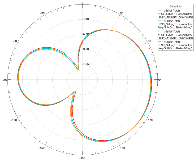
Antenna Gain Pattern, Theta = 90
