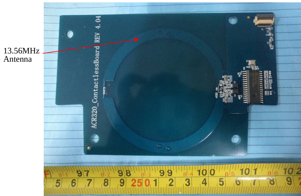
EUT – Contactless Board Top View
