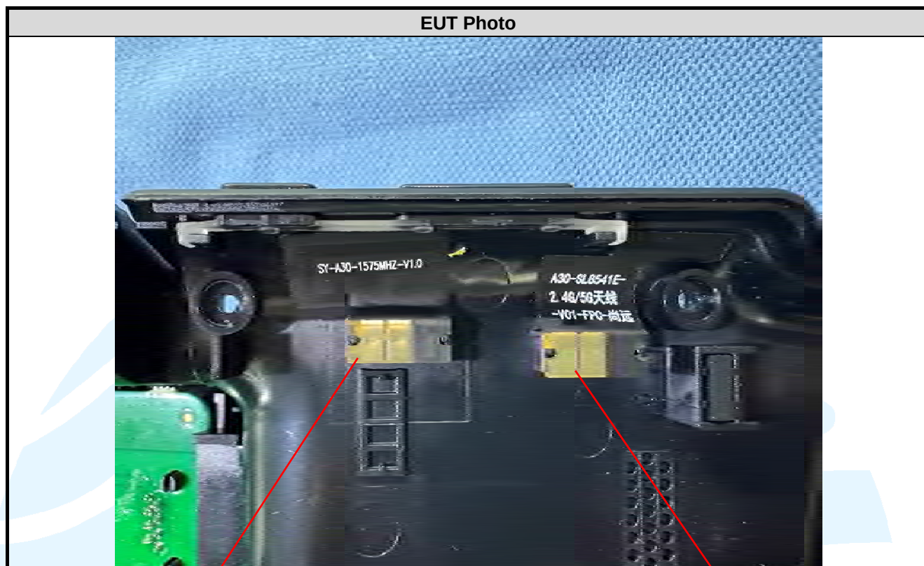
BT/Wi-Fi Antenna
