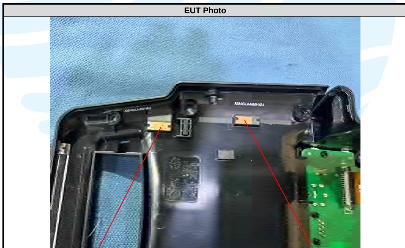
WWAN Main Antenna
