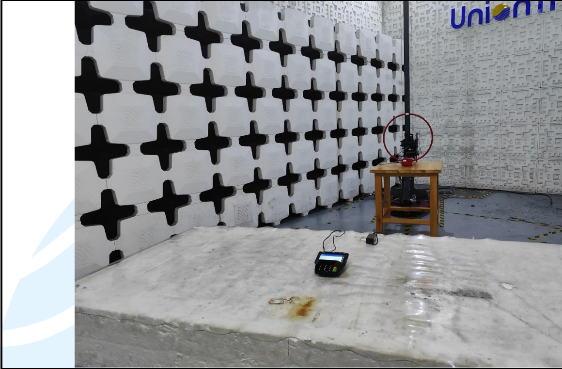
Radiated emission Test Setup (Below 30 MHz)
