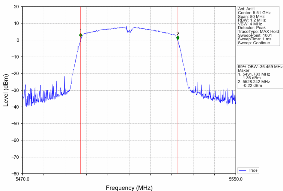
802.11ac(VHT40)_LCH_5510MHz_Ant1_NTNV
