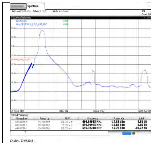
Band12-5MHz-16QAM-23035-25RB#0-PASS
