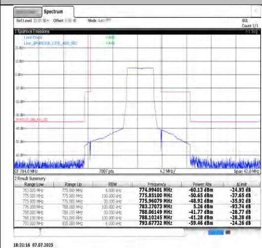
Band13-5MHz-16QAM-23205-1RB#24-PASS
