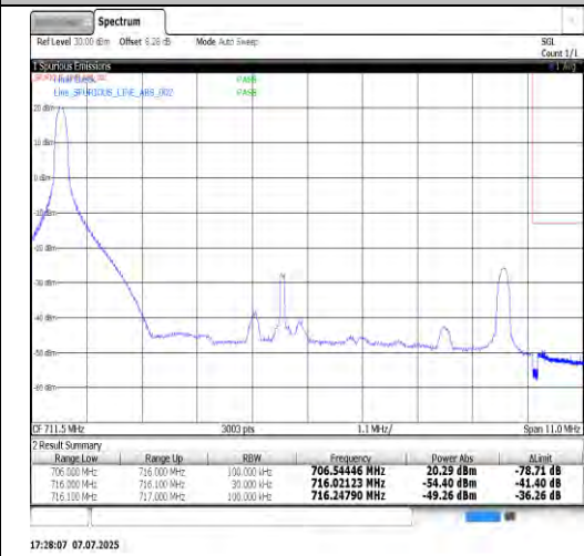
Band12-10MHz-QPSK-23130-50RB#0-PASS
