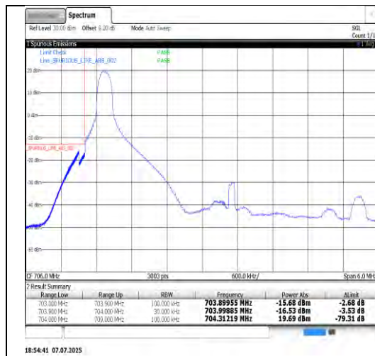
Band17-5MHz-QPSK-23755-25RB#0-PASS
