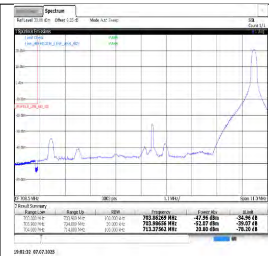
Band17-10MHz-QPSK-23800-1RB#0-PASS
