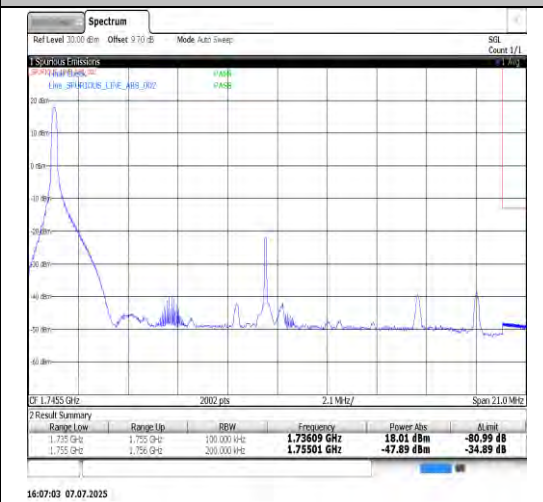
Band4-20MHz-16QAM-20300-100RB#0-PASS
