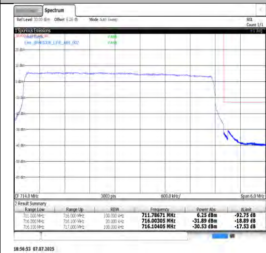
Band17-10MHz-QPSK-23780-1RB#49-PASS
