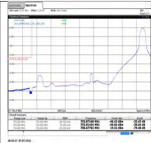
Band17-5MHz-16QAM-23825-1RB#0-PASS
