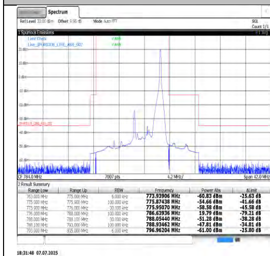
Band13-5MHz-16QAM-23205-1RB#0-PASS
