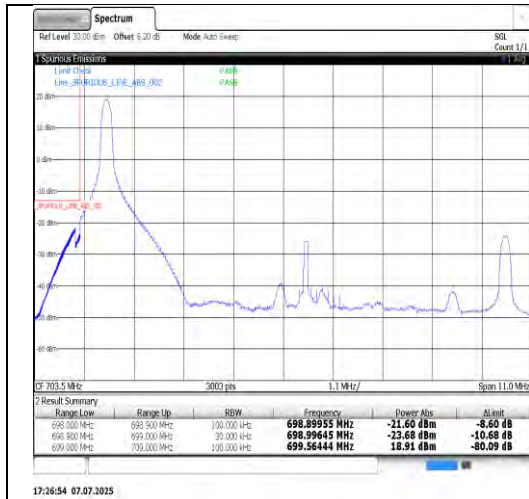
Band12-10MHz-QPSK-23060-50RB#0-PASS
