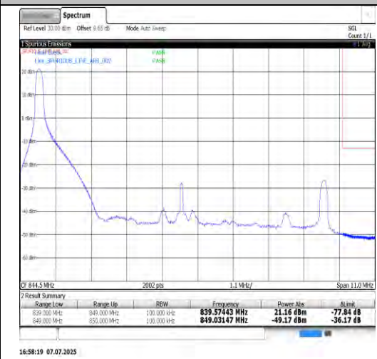
Band5-10MHz-QPSK-20600-50RB#0-PASS
