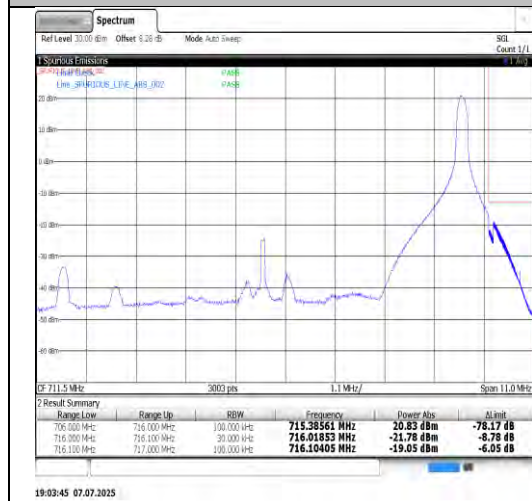
Band17-10MHz-16QAM-23780-1RB#0-PASS
