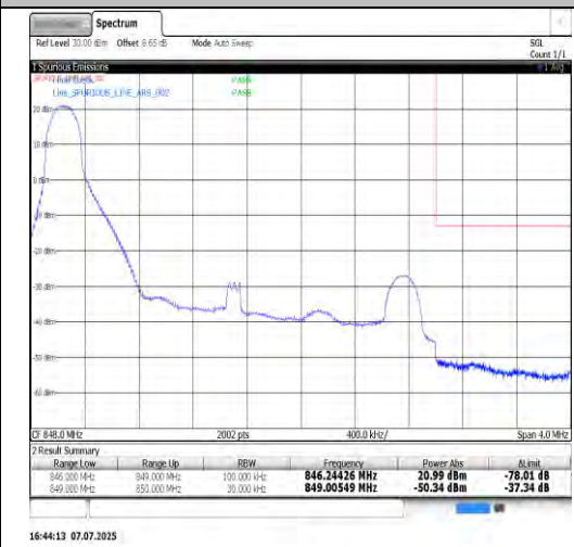
Band5-3MHz-16QAM-20635-15RB#0-PASS
