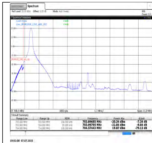
Band17-10MHz-QPSK-23780-50RB#0-PASS
