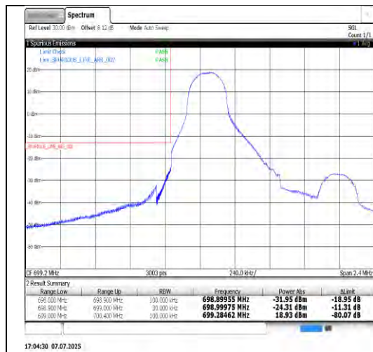
Band12-1.4MHz-QPSK-23017-6RB#0-PASS
