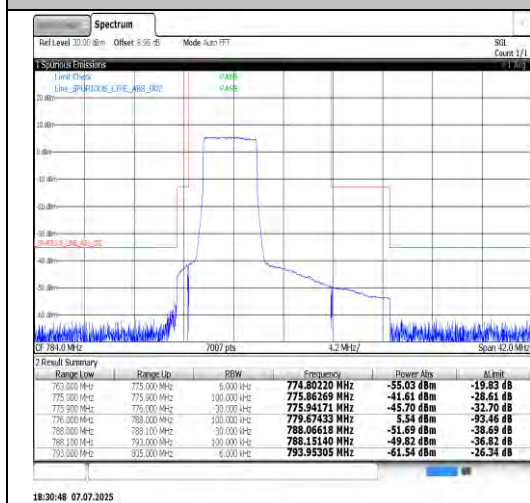
Band13-5MHz-QPSK-23255-1RB#24-PASS
