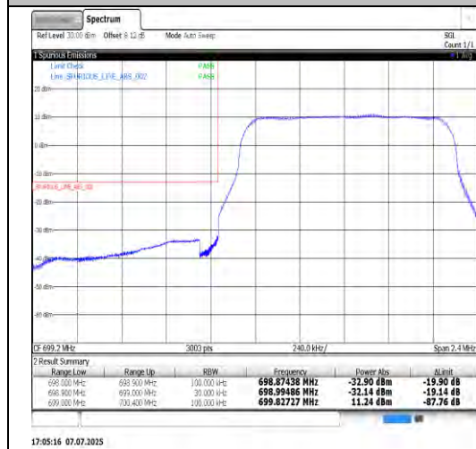
Band12-1.4MHz-QPSK-23173-1RB#5-PASS
