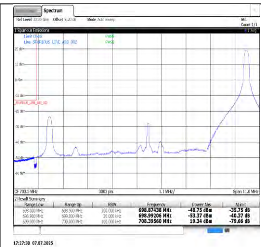
Band12-10MHz-16QAM-23130-1RB#0-PASS
