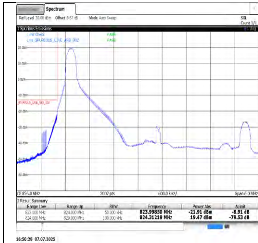
Band5-5MHz-16QAM-20425-25RB#0-PASS
