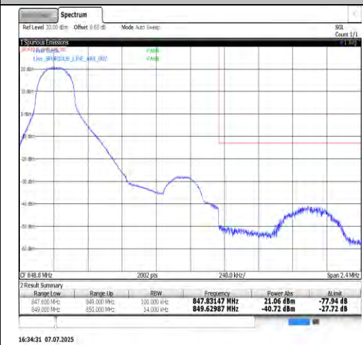
Band5-1.4MHz-16QAM-20643-6RB#0-PASS
