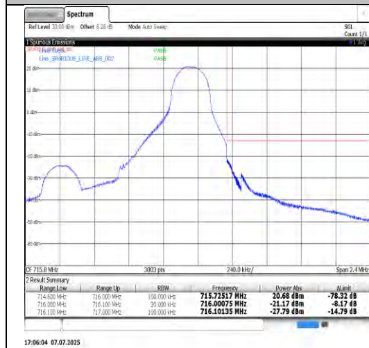
Band12-1.4MHz-16QAM-23017-1RB#0-PASS
