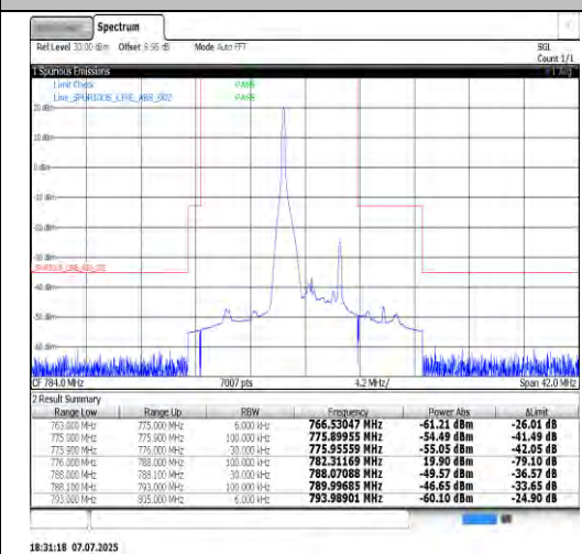
Band13-5MHz-QPSK-23255-25RB#0-PASS
