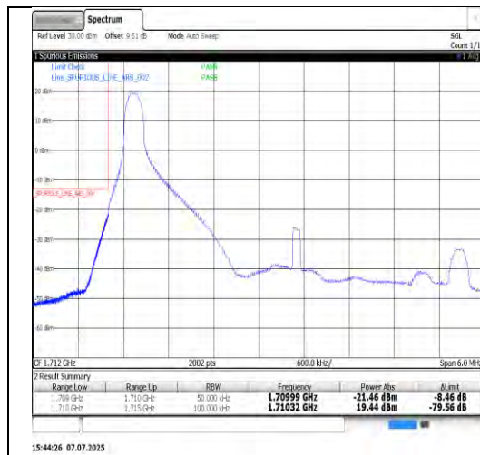
Band4-5MHz-QPSK-19975-25RB#0-PASS
