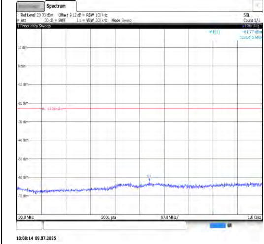
Band2-3MHz-QPSK-18615-1RB#0-1848.5-PASS
