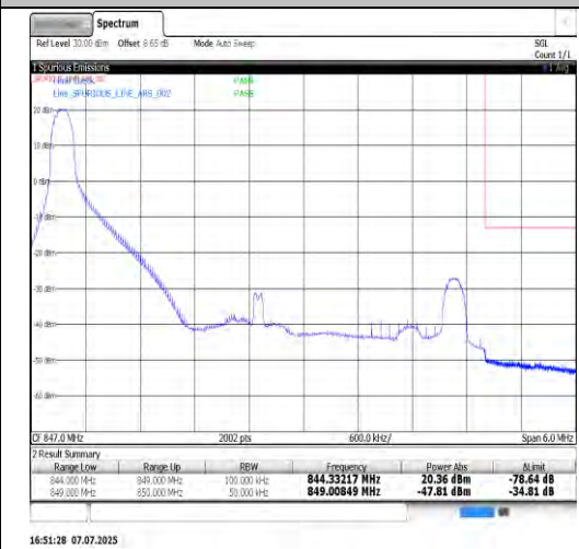
Band5-5MHz-16QAM-20625-25RB#0-PASS
