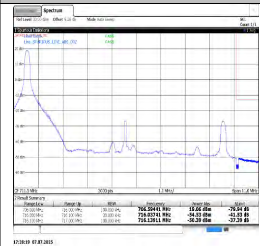
Band12-10MHz-16QAM-23130-50RB#0-PASS
