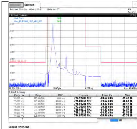
Band13-5MHz-QPSK-23205-25RB#0-PASS
