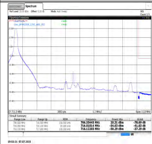
Band17-10MHz-QPSK-23800-50RB#0-PASS
