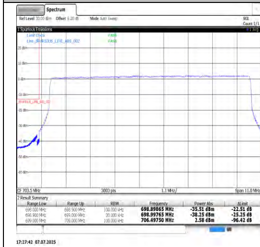
Band12-10MHz-QPSK-23130-1RB#49-PASS
