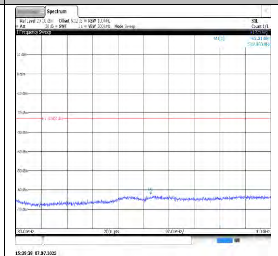
Band4-3MHz-16QAM-19965-1RB#0-1708.5- PASS
