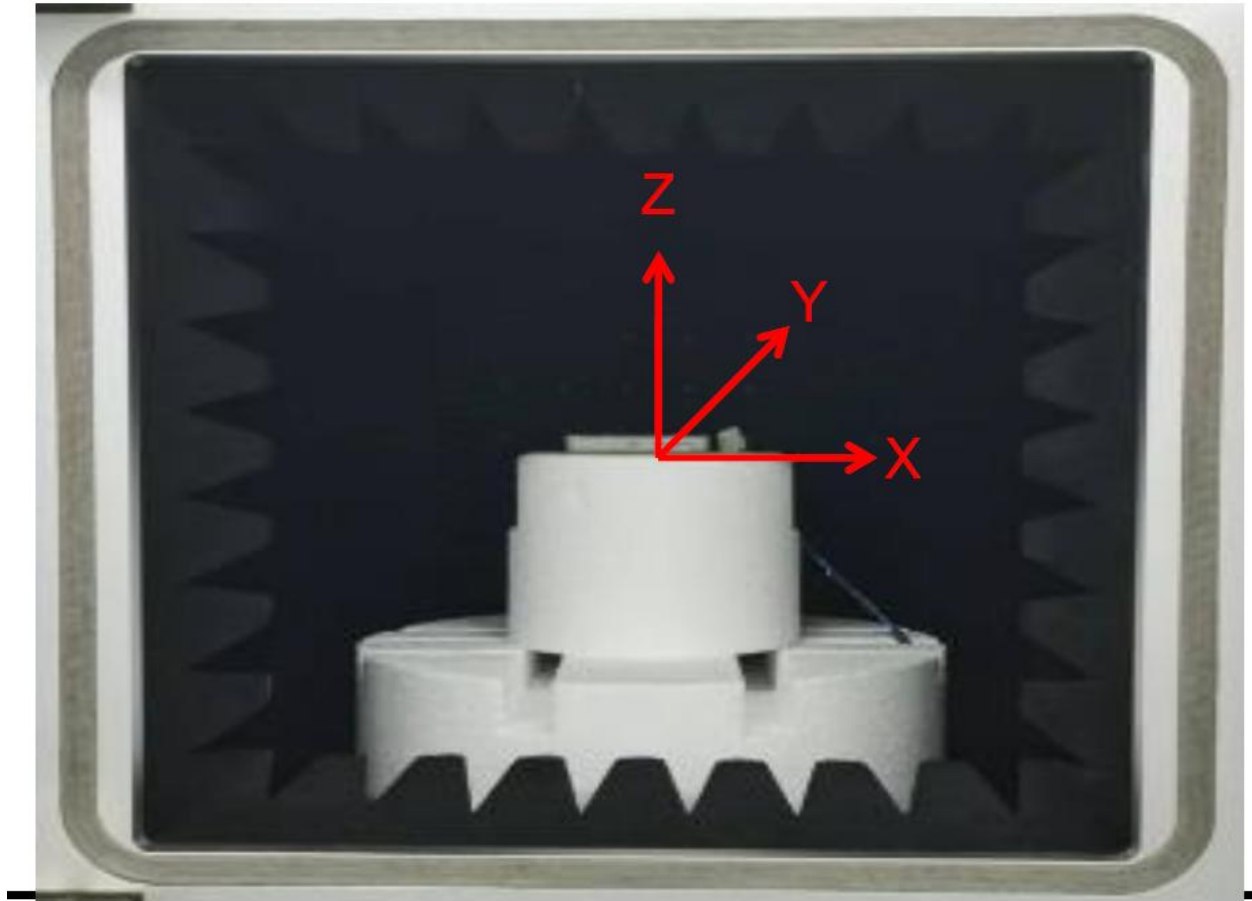
Antenna setup photo
