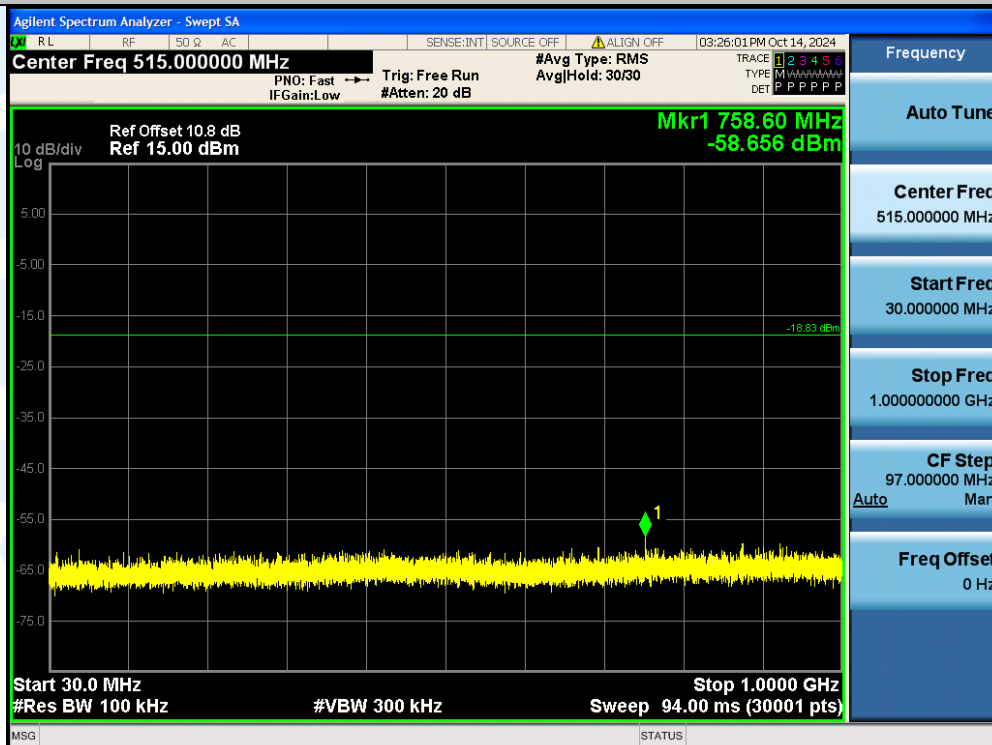
11N40SISO-Ant1-2437-30~1000-PASS
