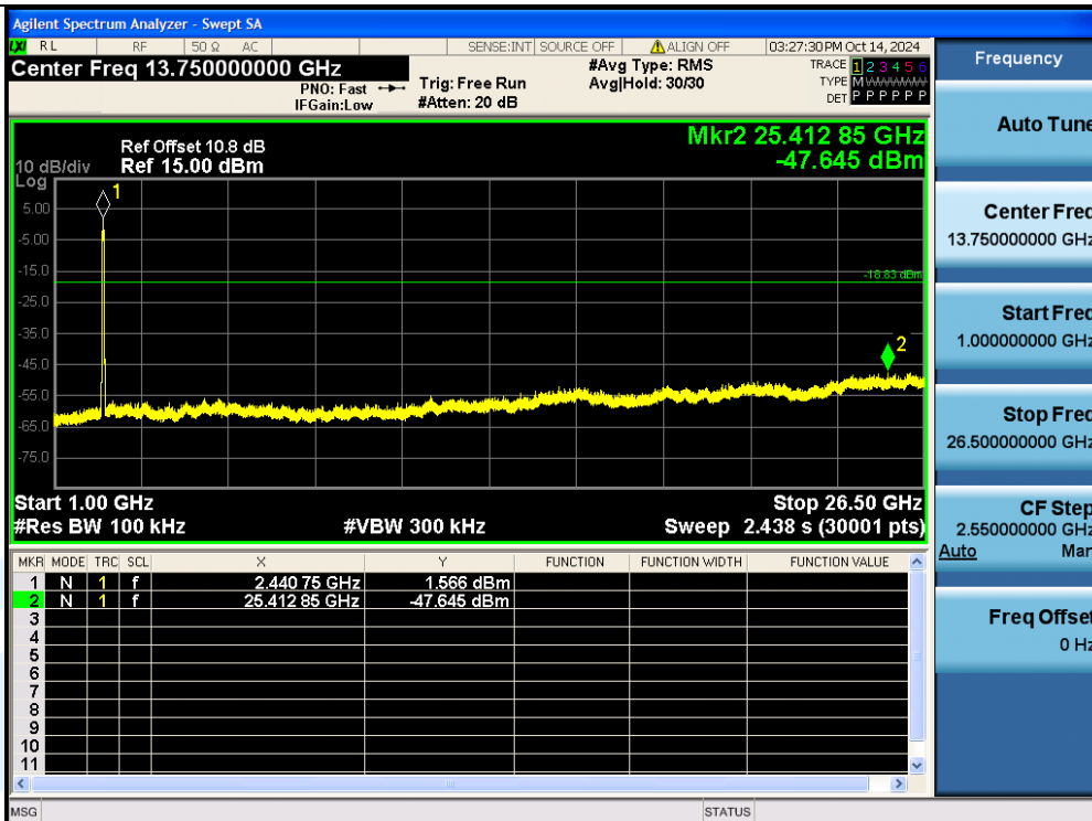
11N40SISO-Ant1-2437-1000~26500-PASS
