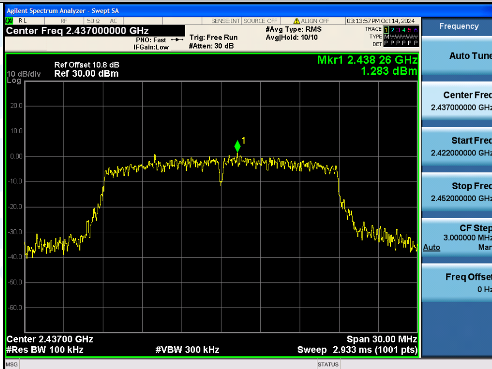
11N20SISO-Ant1-2437-0~Reference-PASS
