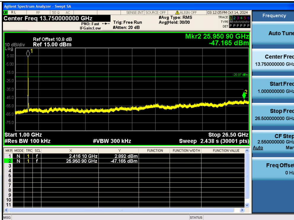
11N20SISO-Ant1-2412-1000~26500-PASS
