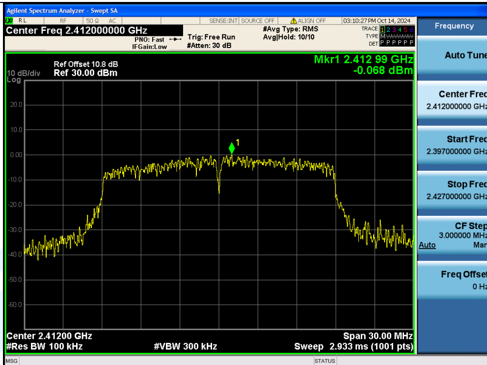
11N20SISO-Ant1-2412-0~Reference-PASS
