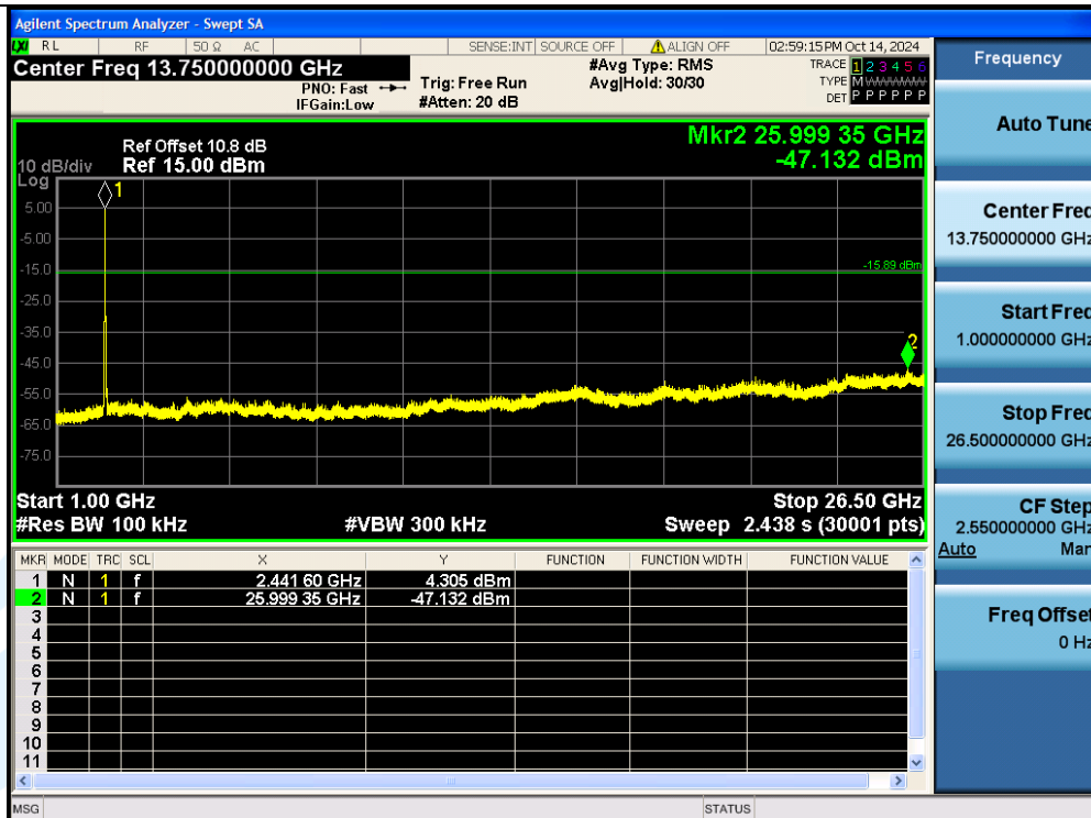
11G-Ant1-2437-1000~26500-PASS
