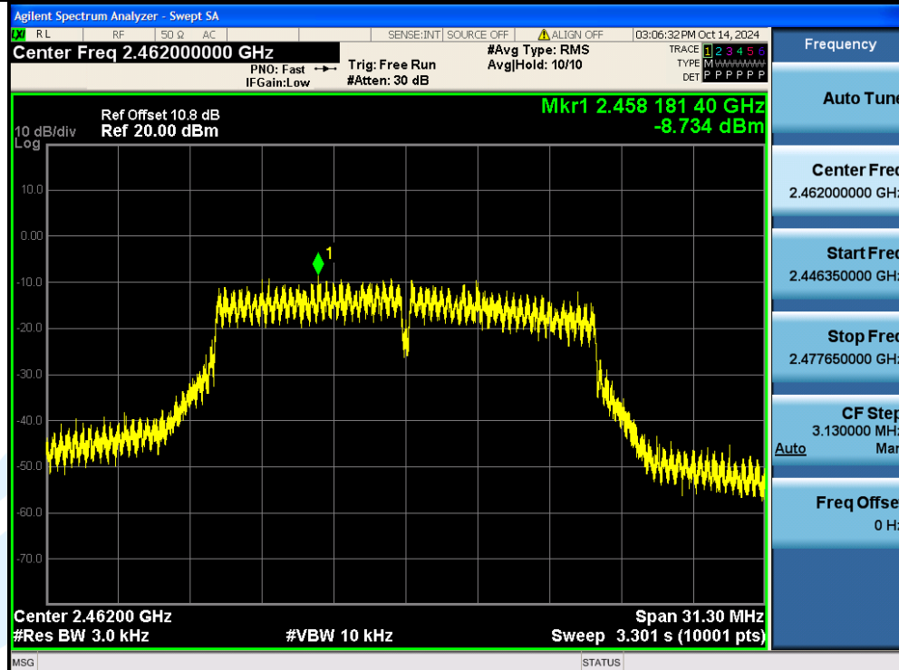
11G-Ant1-2462-PASS
