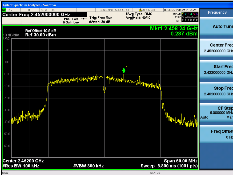
11N40SISO-Ant1-2452-0~Reference-PASS
