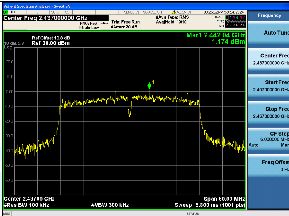
11N40SISO-Ant1-2437-0~Reference-PASS
