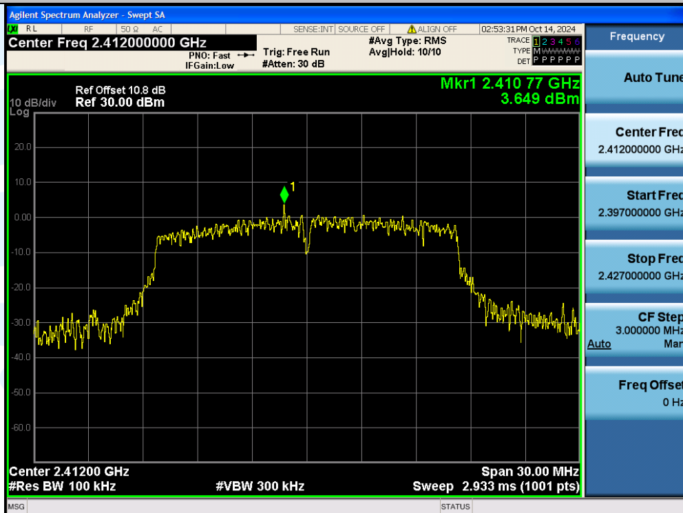
11G-Ant1-2412-0~Reference-PASS
