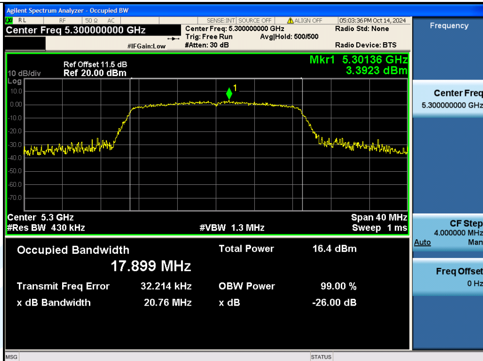
11AC20SISO-Ant1-5300
