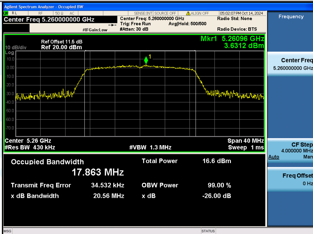
11AC20SISO-Ant1-5260
