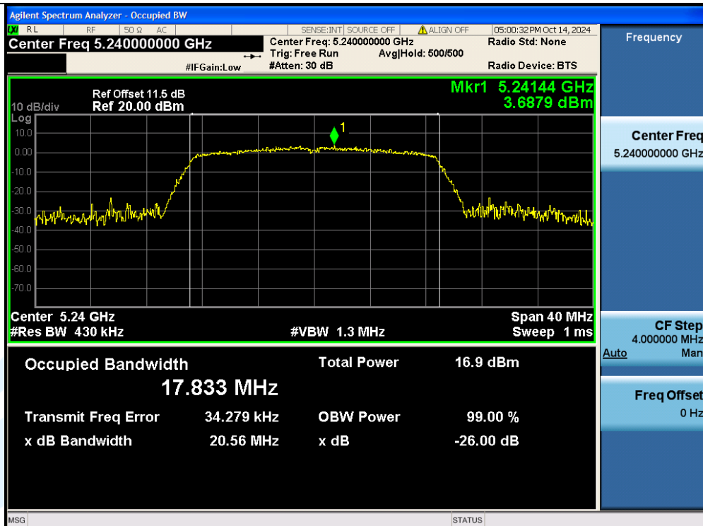
11AC20SISO-Ant1-5240
