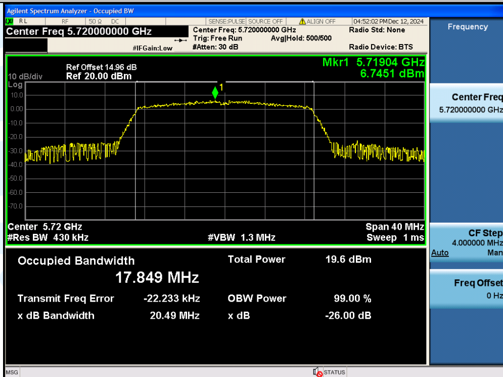
11N20SISO-Ant1-5720
