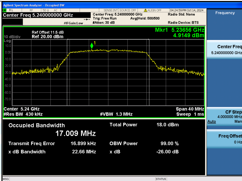
11A-Ant1-5240
