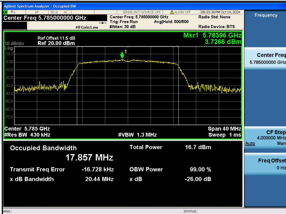
11AC20SISO-Ant1-5785
