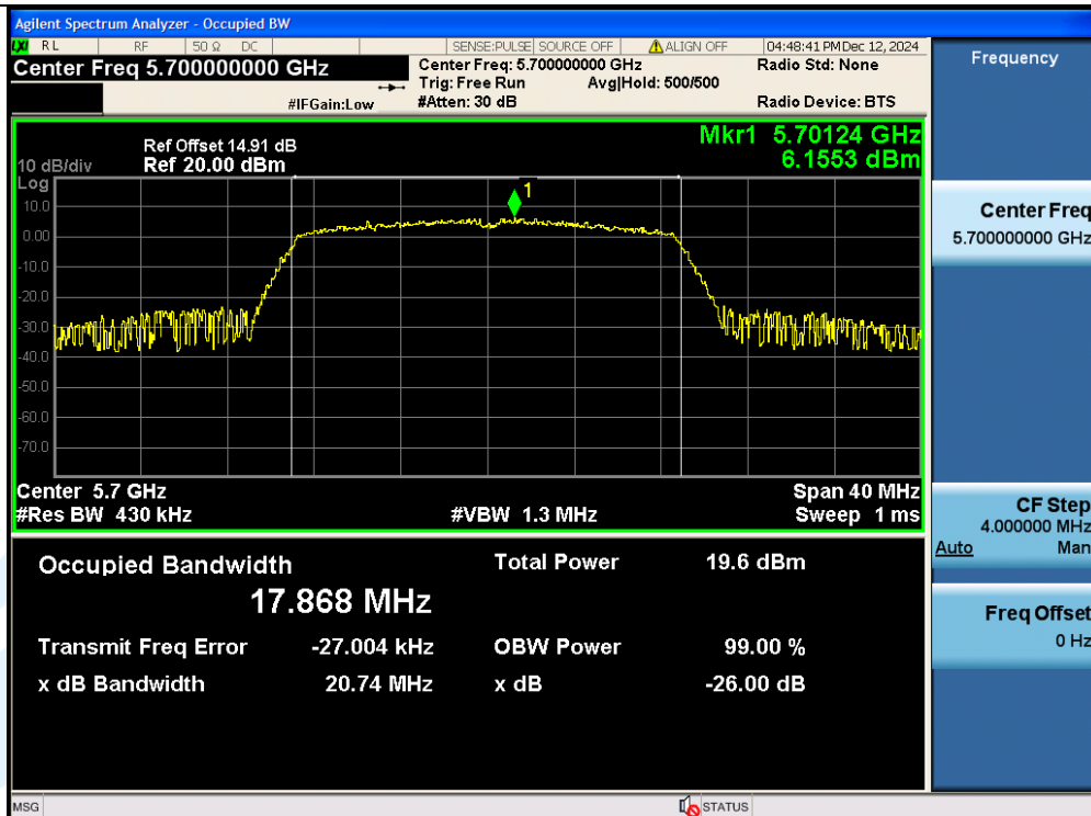
11N20SISO-Ant1-5700
