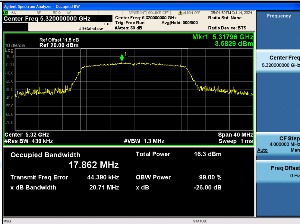
11AC20SISO-Ant1-5320
