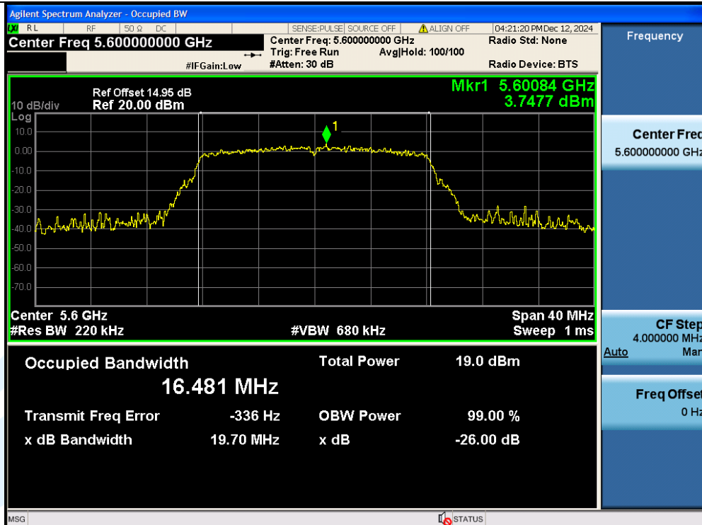
11A-Ant1-5600
