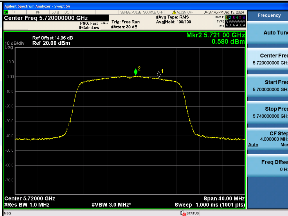
11AC20SISO-Ant1-5720_UNII-2C-PASS
