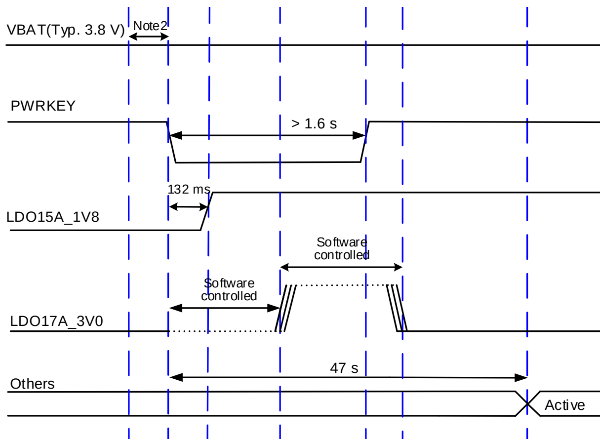
Figure 8: Turn-on Timing
