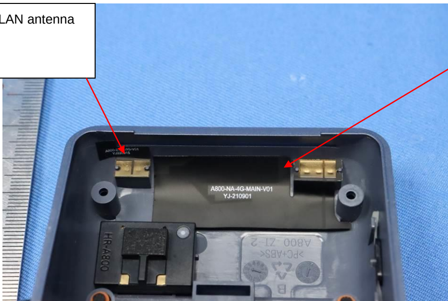
WWAN antenna main
