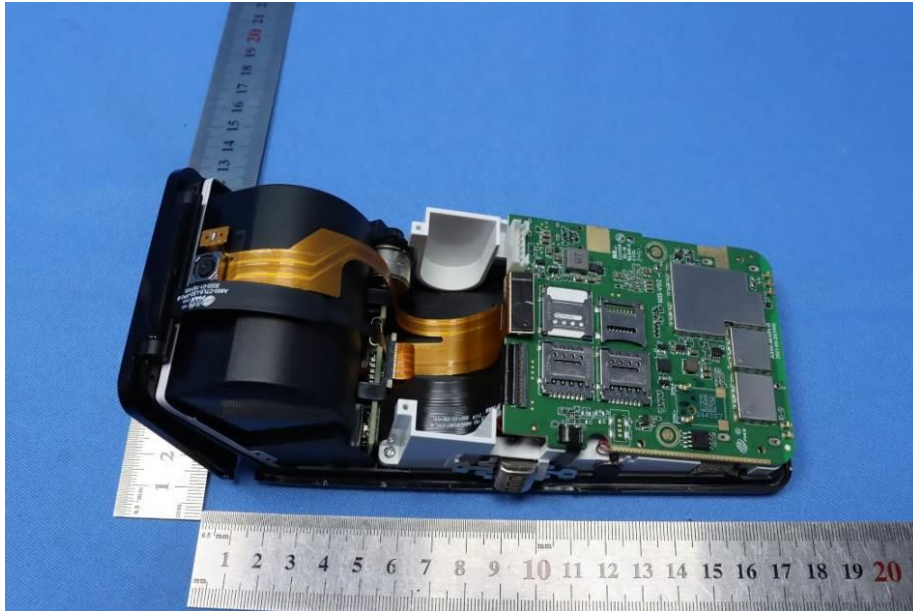
BT/WLAN antenna
