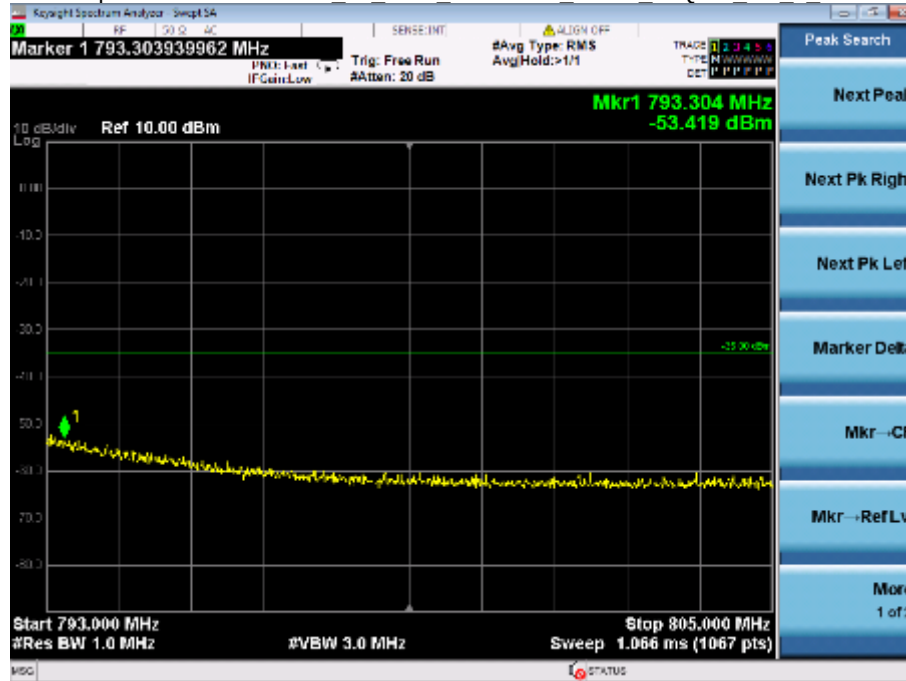
Spurious Emission LTE 13 HCH 784.5MHz NTNv 16QAM RB 12 13
