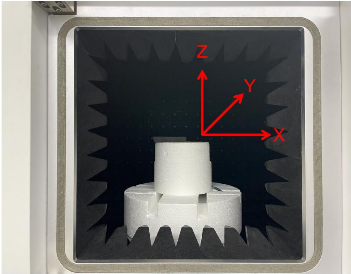
Antenna test setup photo:
