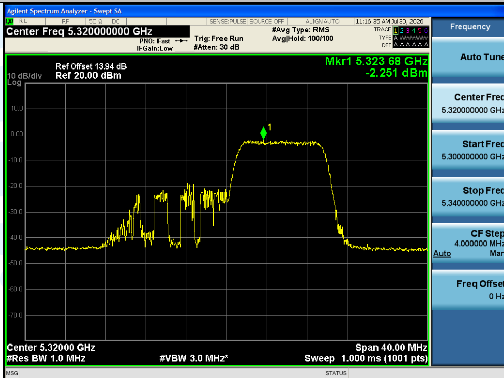
11AX20SISO-Ant1-5320-106Tone-RU54-PASS
