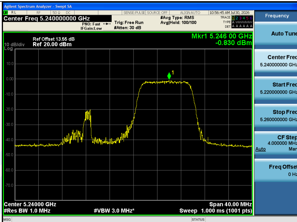
11AX20SISO-Ant1-5240-106Tone-RU54-PASS
