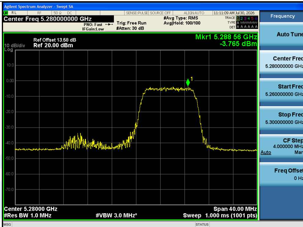
11AX20SISO-Ant1-5280-106Tone-RU54-PASS
