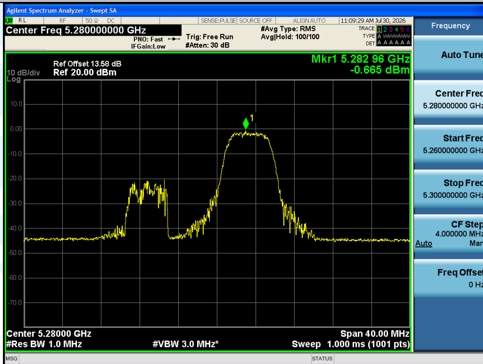
11AX20SISO-Ant1-5280-52Tone-RU39-PASS
