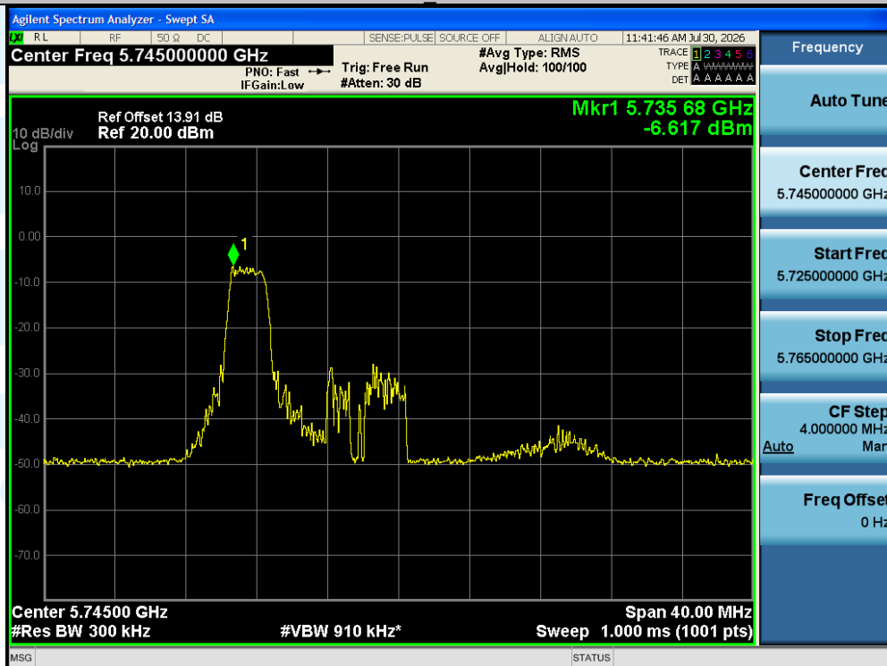
11AX20SISO-Ant1-5745-26Tone-RU0-PASS
