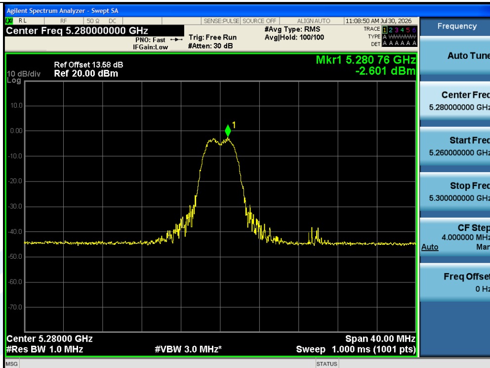
11AX20SISO-Ant1-5280-26Tone-RU4-PASS
