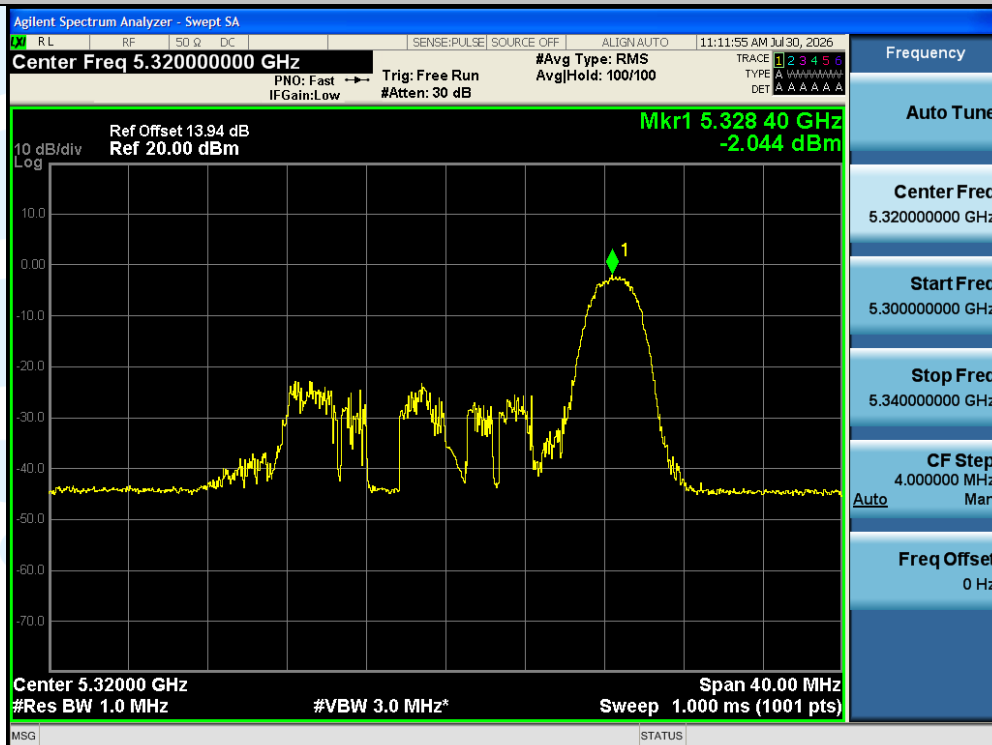
11AX20SISO-Ant1-5320-26Tone-RU8-PASS
