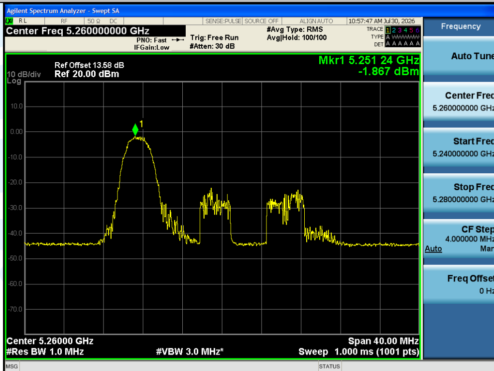
11AX20SISO-Ant1-5260-26Tone-RU0-PASS
