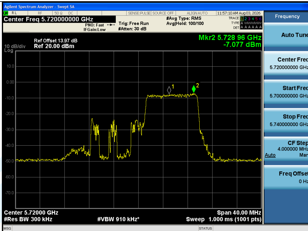
11AX20SISO-Ant1-5720_UNII-3-106Tone-RU54-PASS
