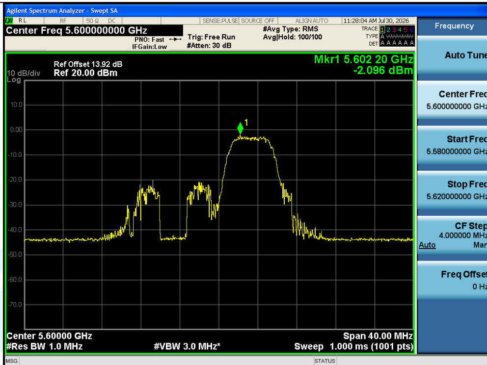
11AX20SISO-Ant1-5600-52Tone-RU39-PASS
