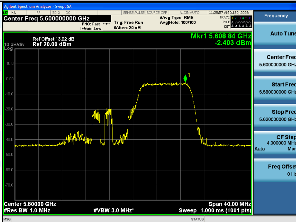
11AX20SISO-Ant1-5600-106Tone-RU54-PASS
