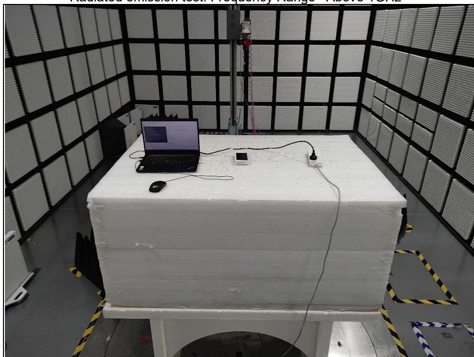
Radiated emission test: Frequency Range < Above 1GHz >
