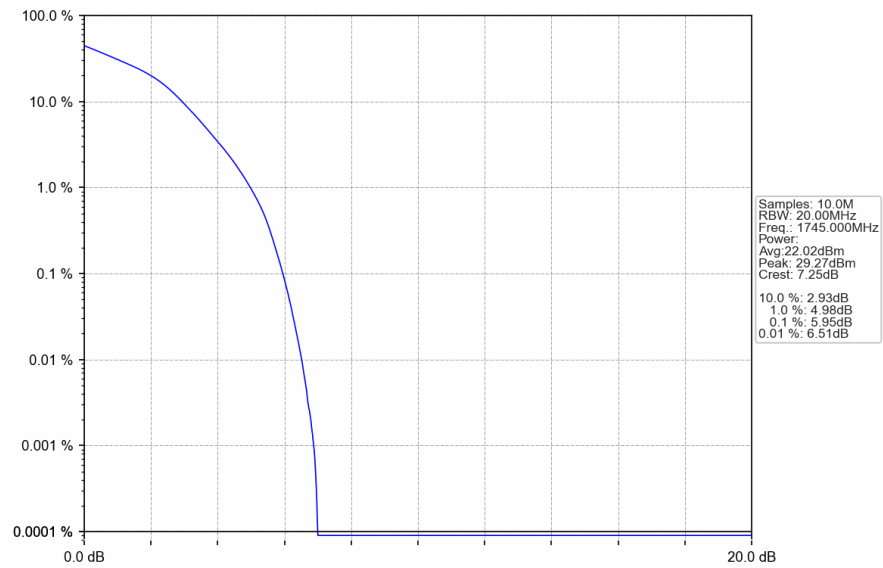
Band4_20MHz_16QAM_HCH_1745MHz_RB_100_0_NTNV
