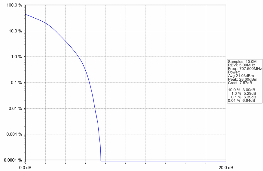
Band12_5MHz_16QAM_MCH_707.5MHz_RB_25_0_NTNV
