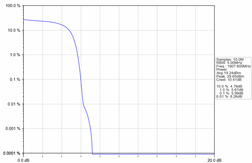
Band2_HSDPA_HCH_1907.6MHz_Subtest 1_NTNV
