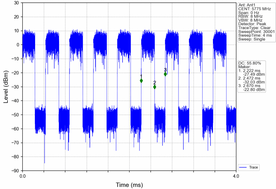
802.11ac(VHT80)_MCH_5775MHz_Ant1_NTNV
