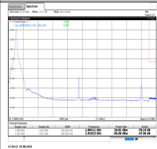
Band2-20MHz-16QAM-19100-100RB#0-PASS
