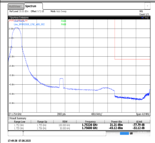
Band4-3MHz-QPSK-20385-15RB#0-PASS
