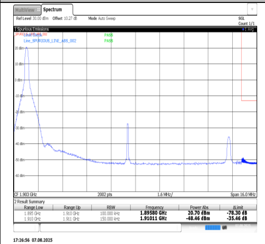
Band2-15MHz-16QAM-19125-75RB#0-PASS
