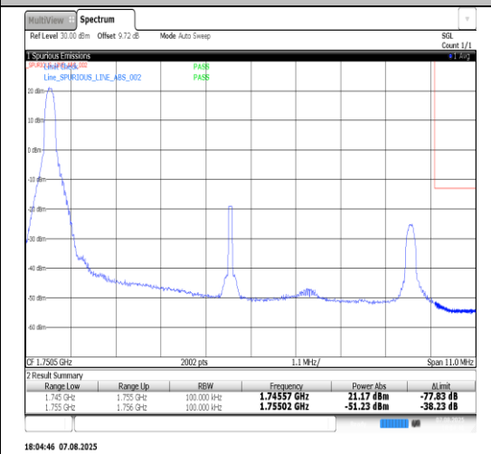
Band4-10MHz-QPSK-20350-50RB#0-PASS
