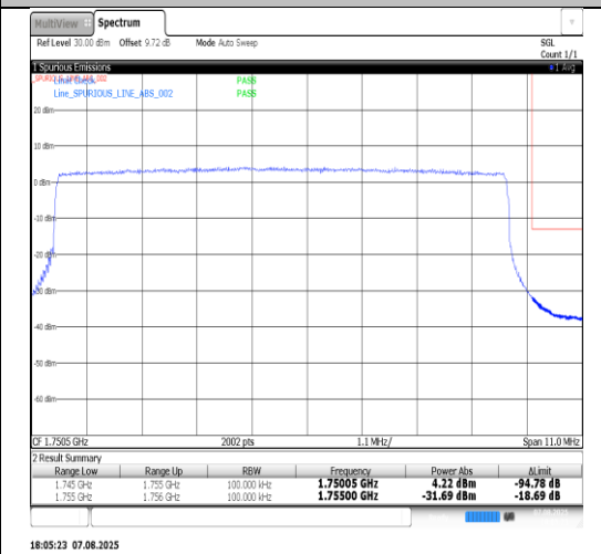
Band4-10MHz-16QAM-20000-1RB#49-PASS
