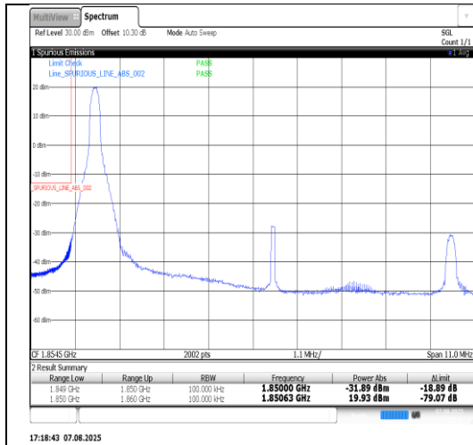
Band2-10MHz-16QAM-18650-50RB#0-PASS
