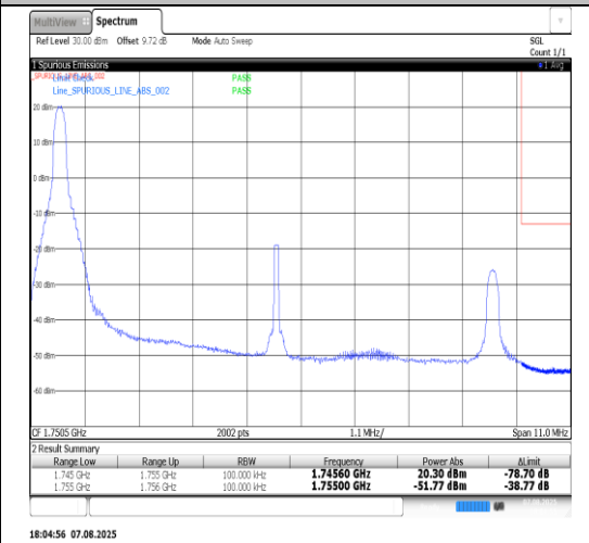
Band4-10MHz-16QAM-20350-50RB#0-PASS
