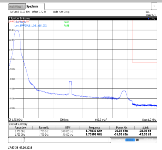
Band4-5MHz-16QAM-20375-25RB#0-PASS
