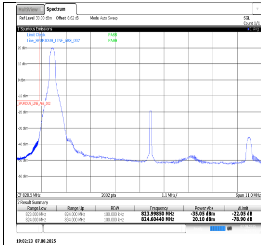
Band5-10MHz-16QAM-20450-50RB#0-PASS
