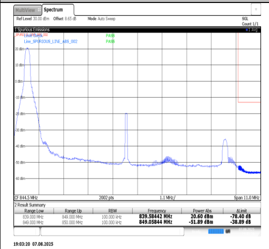
Band5-10MHz-16QAM-20600-50RB#0-PASS
