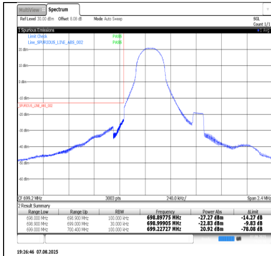
Band12-1.4MHz-QPSK-23017-6RB#0-PASS
