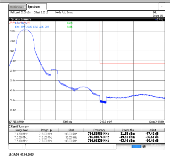
Band12-1.4MHz-QPSK-23173-6RB#0-PASS
