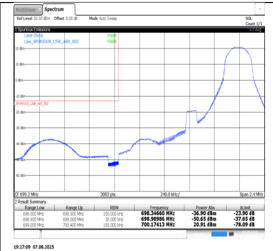
Band12-1.4MHz-QPSK-23173-1RB#0-PASS
