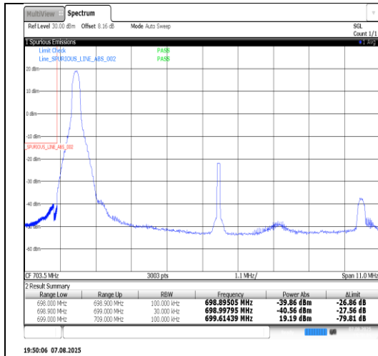
Band12-10MHz-16QAM-23060-50RB#0-PASS
