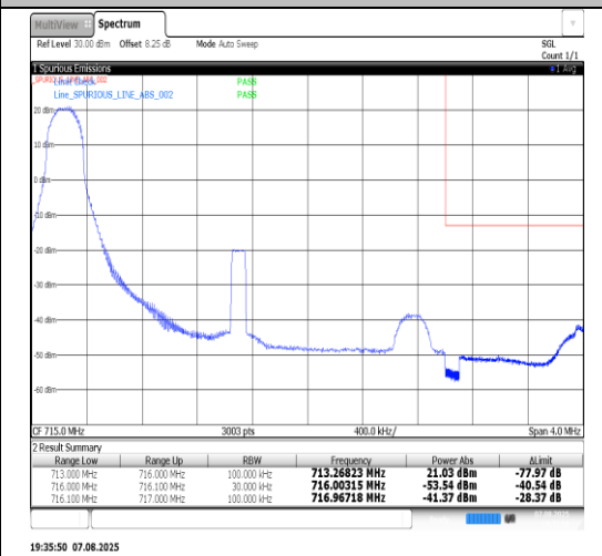
Band12-3MHz-16QAM-23165-15RB#0-PASS
