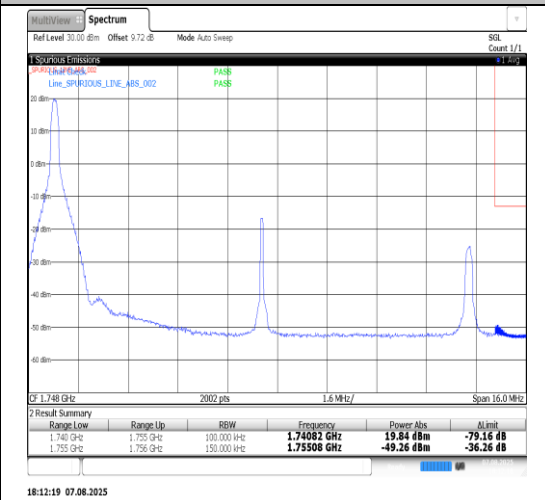
Band4-15MHz-16QAM-20325-75RB#0-PASS
