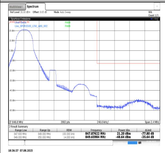
Band5-1.4MHz-16QAM-20643-6RB#0-PASS
