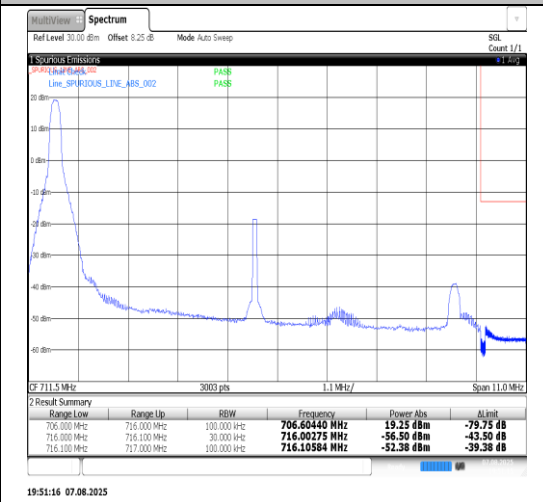
Band12-10MHz-16QAM-23130-50RB#0-PASS
