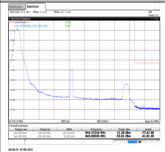
Band5-5MHz-16QAM-20625-25RB#0-PASS
