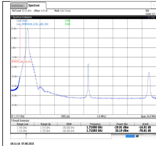
Band4-15MHz-16QAM-20025-75RB#0-PASS
