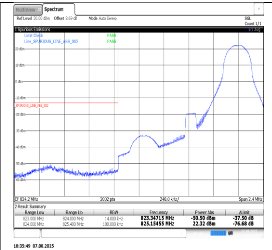
Band5-1.4MHz-QPSK-20643-1RB#0-PASS
