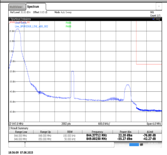
Band5-5MHz-QPSK-20625-25RB#0-PASS
