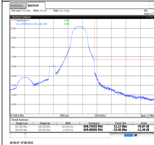
Band5-1.4MHz-16QAM-20407-1RB#0-PASS
