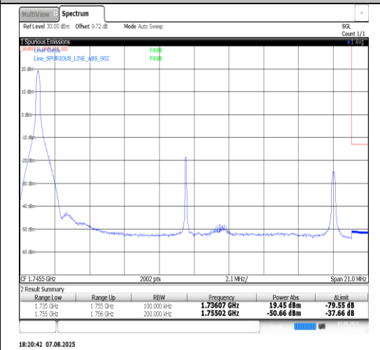
Band4-20MHz-16QAM-20300-100RB#0-PASS
