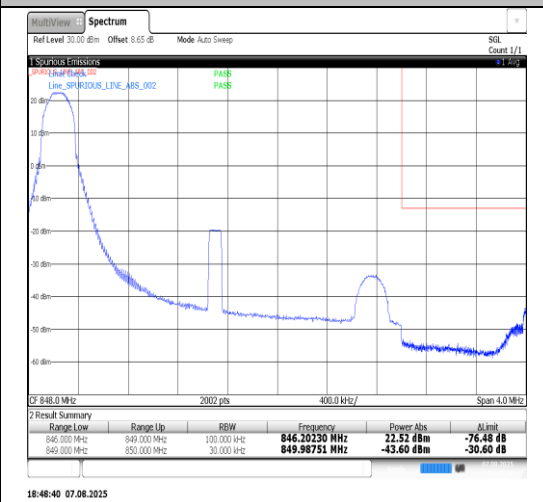
Band5-3MHz-QPSK-20635-15RB#0-PASS
