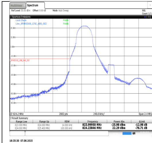
Band5-1.4MHz-QPSK-20407-6RB#0-PASS
