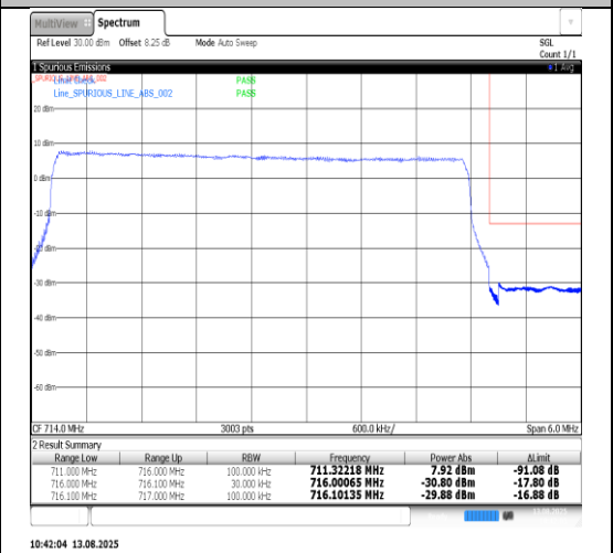
Band17-10MHz-QPSK-23780-1RB#49-PASS
