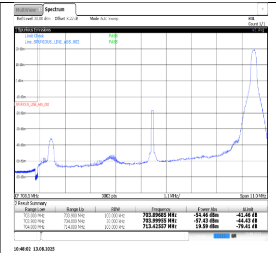
Band17-10MHz-16QAM-23800-1RB#0-PASS
