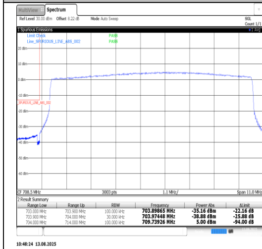
Band17-10MHz-16QAM-23800-1RB#49-PASS
