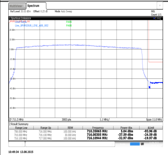
Band17-10MHz-16QAM-23800-50RB#0-PASS
