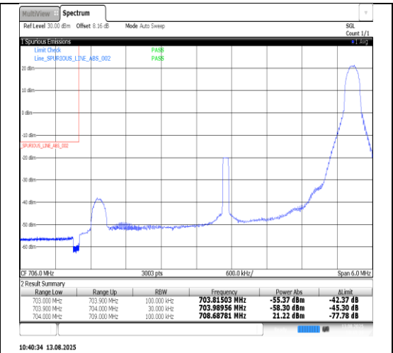
Band17-5MHz-16QAM-23825-1RB#0-PASS
