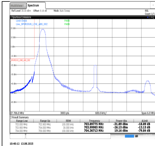
Band17-5MHz-16QAM-23755-25RB#0-PASS
