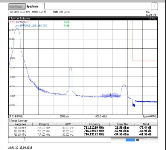
Band17-5MHz-16QAM-23825-25RB#0-PASS
