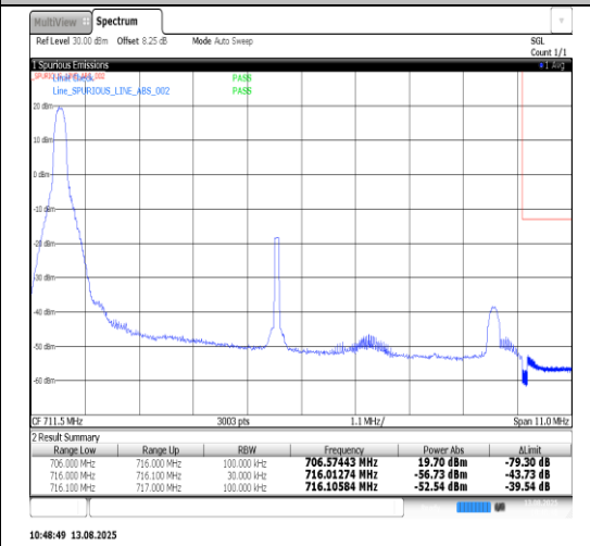
Band17-10MHz-16QAM-23800-50RB#0-PASS
