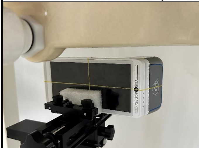
Left Side of EUT with 1.5 cm Gap
