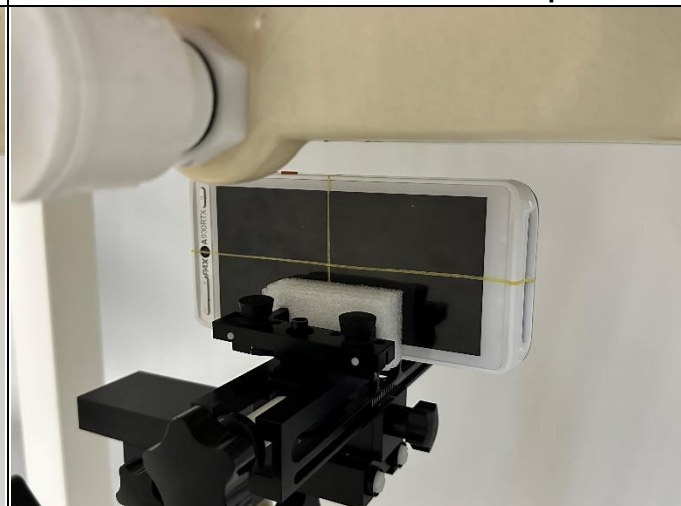
Right Side of EUT with 1.5 cm Gap
