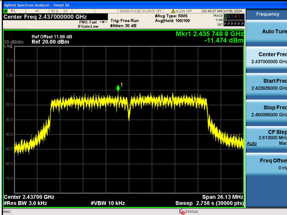
11N20SISO-Ant1-2437-PASS
