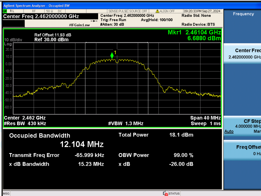
11B-Ant1-2462
