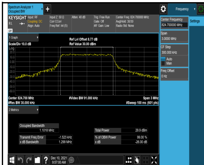
Band5-1.4MHz-QPSK-20407-6RB#0
