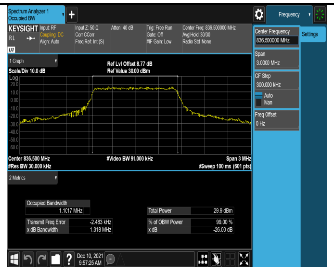
Band5-1.4MHz-QPSK-20525-6RB#0
