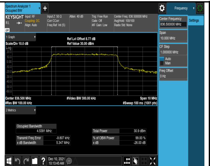
Band5-5MHz-QPSK-20525-25RB#0
