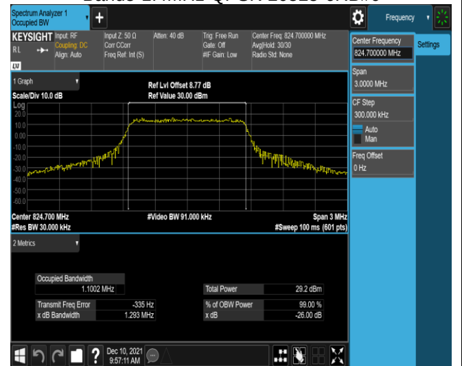
Band5-1.4MHz-16QAM-20407-6RB#0
