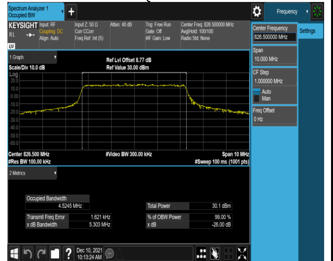
Band5-5MHz-16QAM-20425-25RB#0
