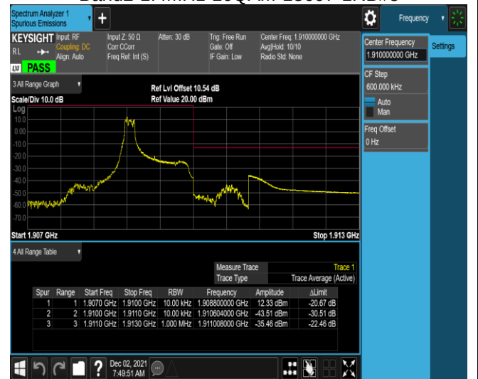
Band2-1.4MHz-16QAM-19193-1RB#0
