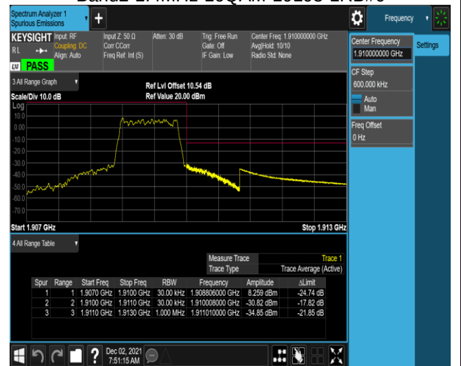
Band2-1.4MHz-16QAM-19193-6RB#0
