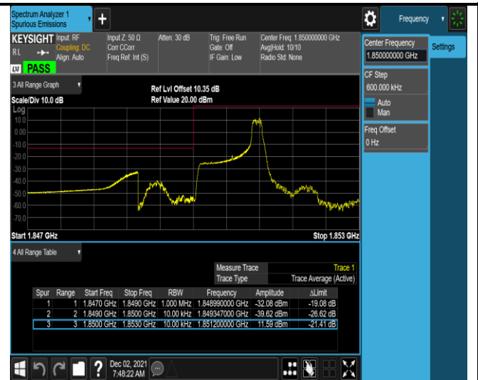
Band2-1.4MHz-16QAM-18607-1RB#5
