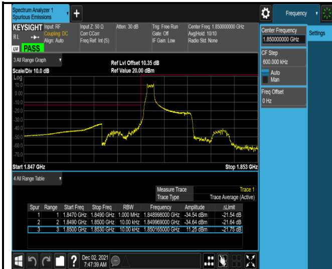
Band2-1.4MHz-16QAM-18607-1RB#0
