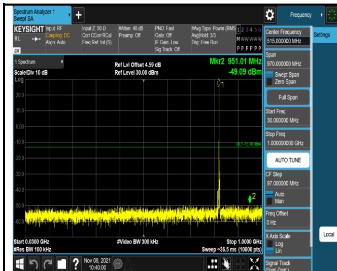
Band5-1.4MHz-QPSK-20407-1RB#0- Range1:30~1000MHz
