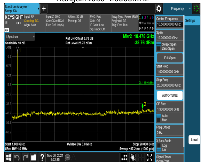
Band4-1.4MHz-16QAM-20393-1RB#0- Range2:1000~20000MHz
