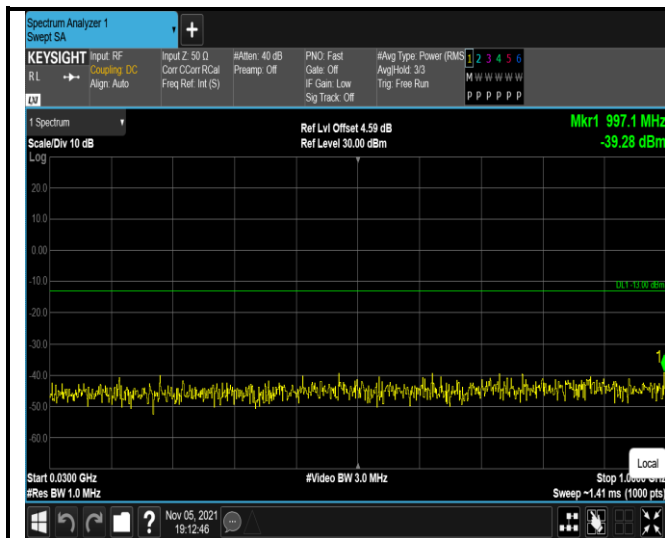
Band2-20MHz-16QAM-18700-1RB#0- Range1:30~1000MHz
