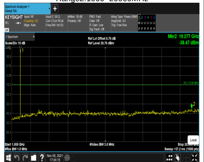
Band2-1.4MHz-16QAM-18900-1RB#0- Range2:1000~20000MHz
