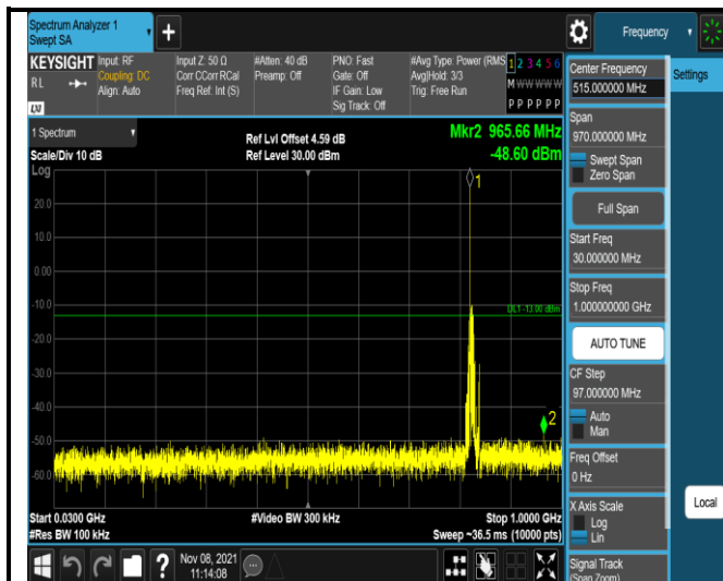
Band5-10MHz-QPSK-20450-1RB#0- Range1:30~1000MHz
