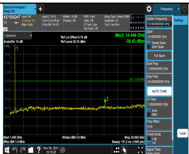
Band4-20MHz-16QAM-20050-1RB#0- Range2:1000~20000MHz
