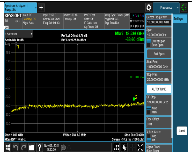
Band4-1.4MHz-16QAM-19957-1RB#0- Range2:1000~20000MHz
