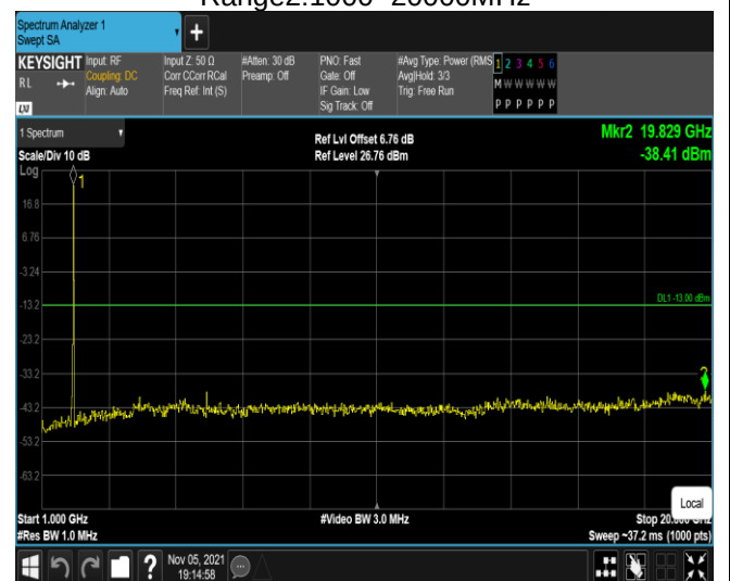
Band2-20MHz-16QAM-19100-1RB#0- Range2:1000~20000MHz
