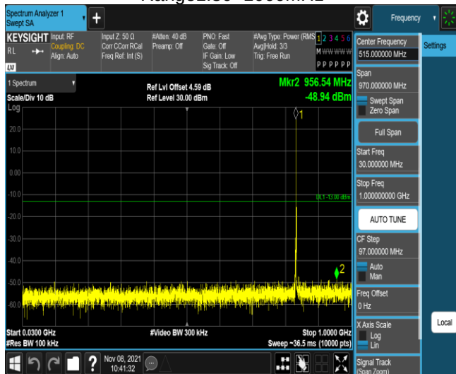
Band5-1.4MHz-16QAM-20525-1RB#0- Range1:30~1000MHz
