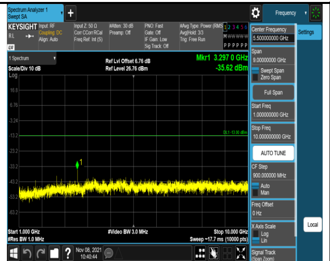
Band5-1.4MHz-16QAM-20407-1RB#0- Range2:1000~10000MHz
