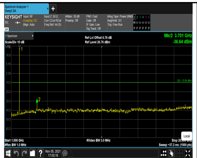
Band2-1.4MHz-16QAM-18607-1RB#0- Range2:1000~20000MHz
