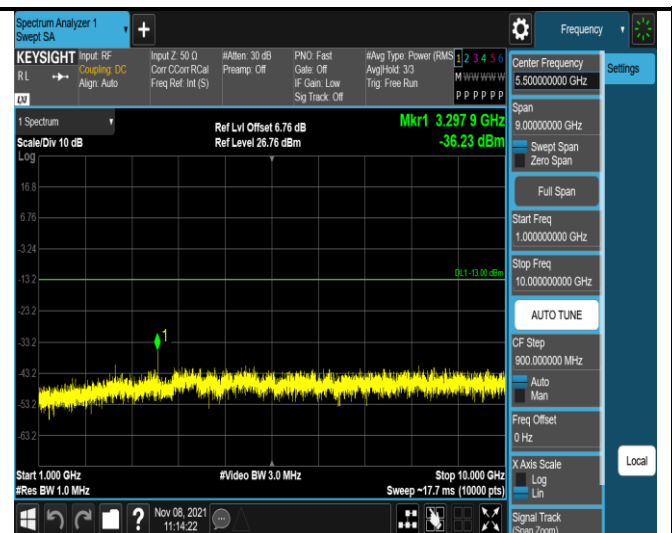
Band5-10MHz-QPSK-20450-1RB#0- Range2:1000~10000MHz
