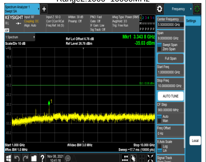
Band5-1.4MHz-QPSK-20525-1RB#0- Range2:1000~10000MHz
