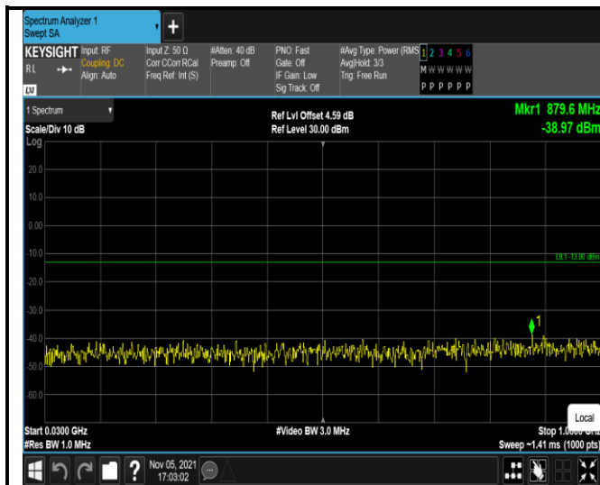
Band2-1.4MHz-16QAM-18607-1RB#0- Range1:30~1000MHz
