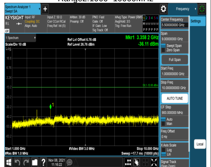
Band5-10MHz-QPSK-20600-1RB#0- Range2:1000~10000MHz
