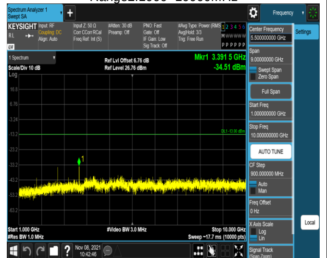
Band5-1.4MHz-16QAM-20643-1RB#0- Range2:1000~10000MHz
