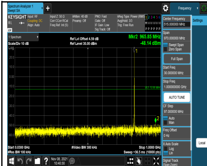
Band5-1.4MHz-16QAM-20407-1RB#0- Range1:30~1000MHz
