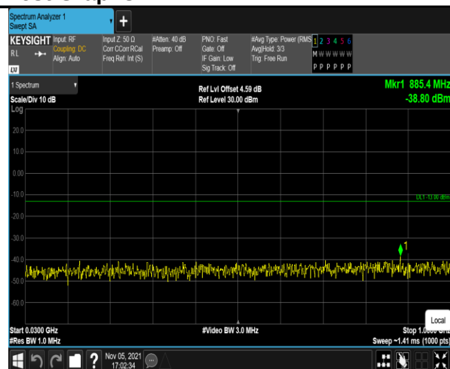
Band2-1.4MHz-QPSK-18607-1RB#0- Range1:30~1000MHz
