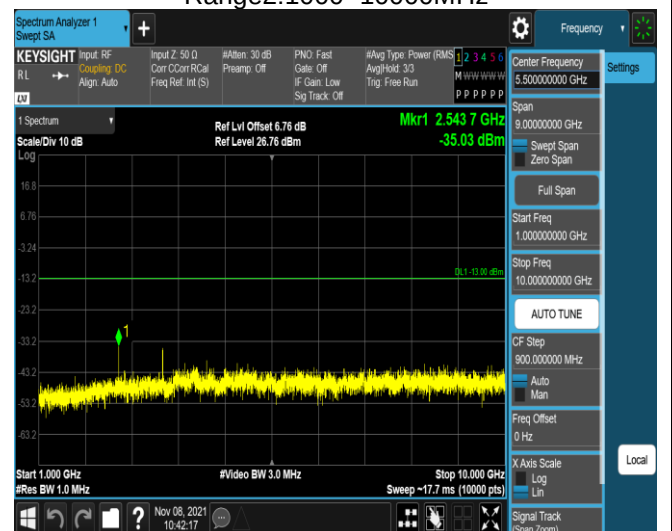
Band5-1.4MHz-QPSK-20643-1RB#0- Range2:1000~10000MHz
