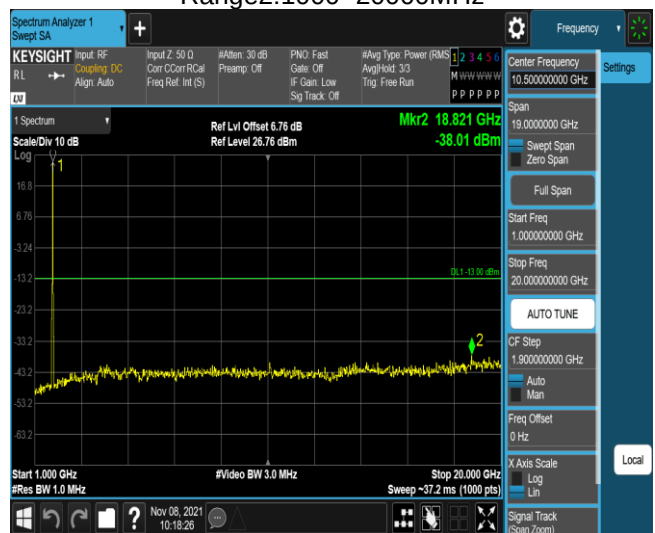
Band4-20MHz-16QAM-20300-1RB#0- Range2:1000~20000MHz
