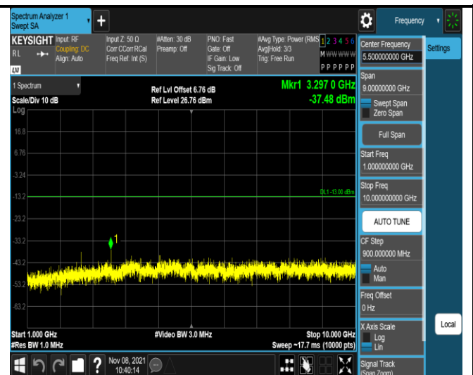
Band5-1.4MHz-QPSK-20407-1RB#0- Range2:1000~10000MHz
