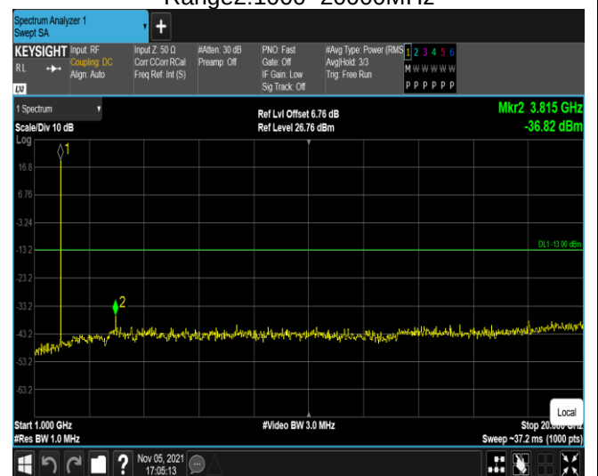
Band2-1.4MHz-16QAM-19193-1RB#0- Range2:1000~20000MHz
