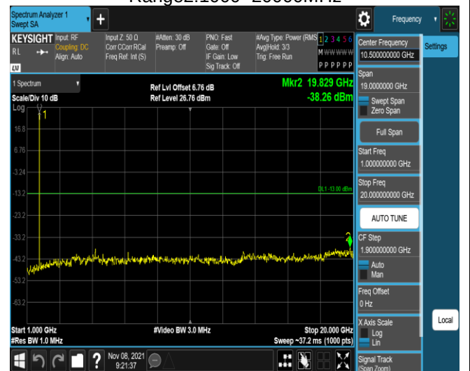
Band4-1.4MHz-16QAM-20175-1RB#0- Range2:1000~20000MHz
