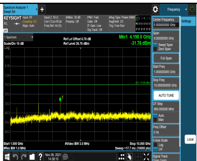
Band12-10MHz-16QAM-23060-1RB#0- Range2:1000~10000MHz
