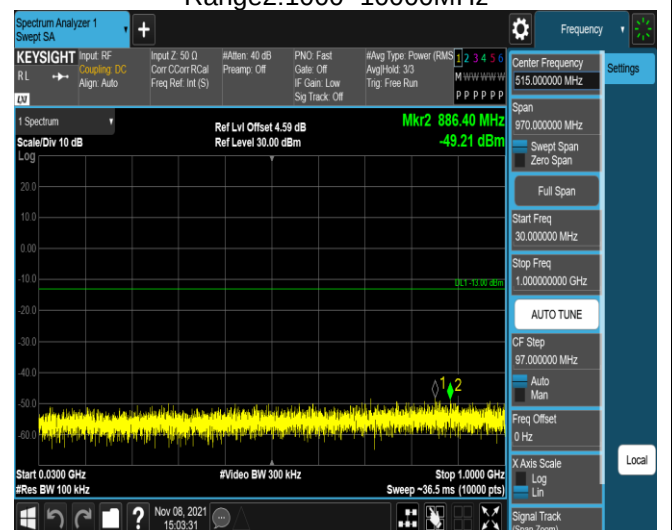
Band13-5MHz-16QAM-23255-1RB#0- Range1:30~1000MHz
