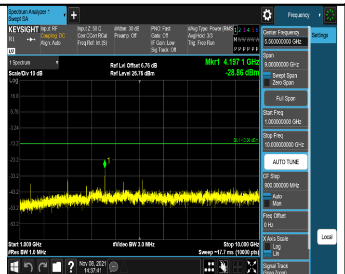
Band12-10MHz-QPSK-23060-1RB#0- Range2:1000~10000MHz
