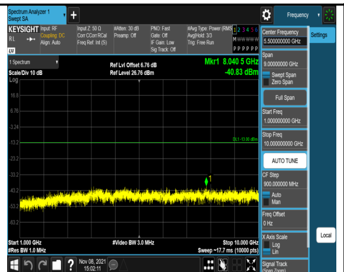
Band13-5MHz-16QAM-23230-1RB#0- Range2:1000~10000MHz
