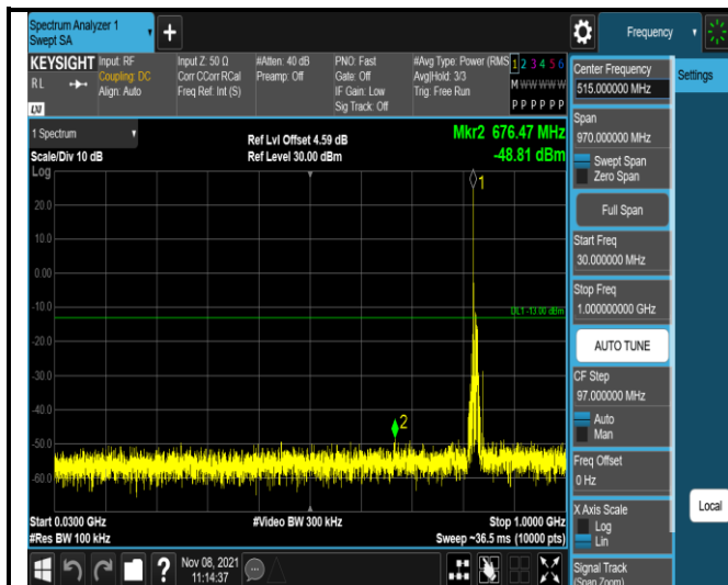
Band5-10MHz-16QAM-20450-1RB#0- Range1:30~1000MHz
