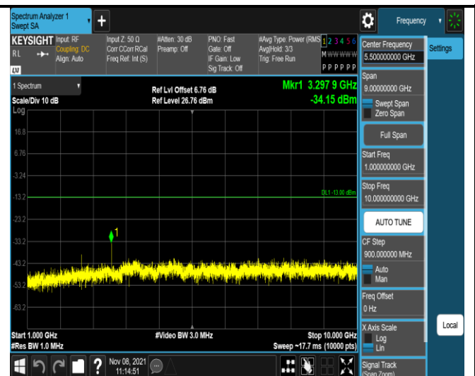
Band5-10MHz-16QAM-20450-1RB#0- Range2:1000~10000MHz
