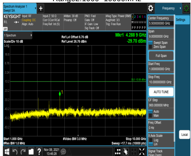
Band12-1.4MHz-QPSK-23173-1RB#0- Range2:1000~10000MHz
