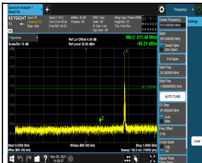
Band13-5MHz-QPSK-23205-1RB#0- Range1:30~1000MHz
