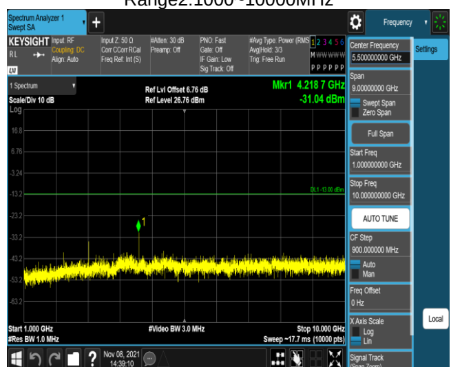
Band12-10MHz-16QAM-23095-1RB#0- Range2:1000~10000MHz
