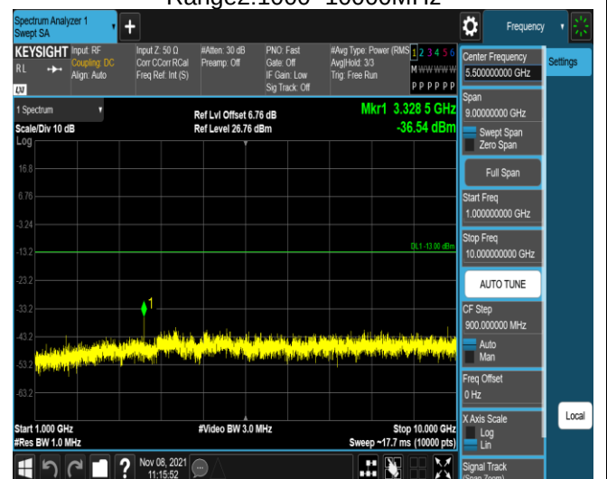
Band5-10MHz-16QAM-20525-1RB#0- Range2:1000~10000MHz
