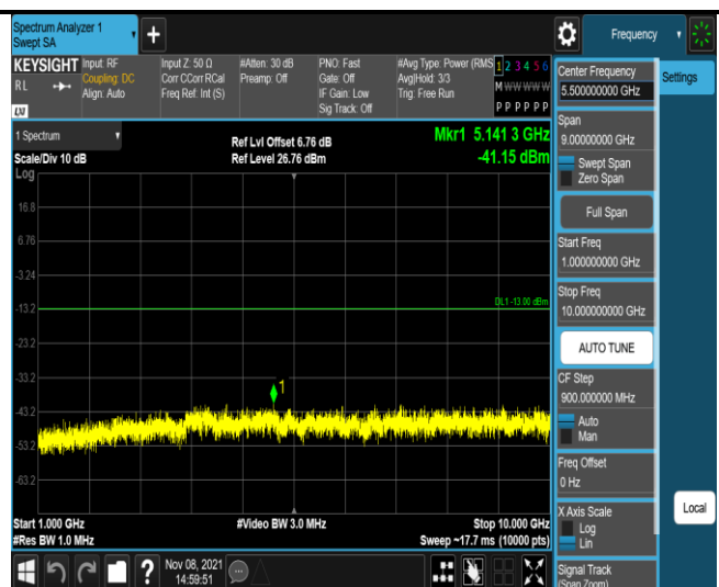
Band13-5MHz-QPSK-23205-1RB#0- Range2:1000~10000MHz
