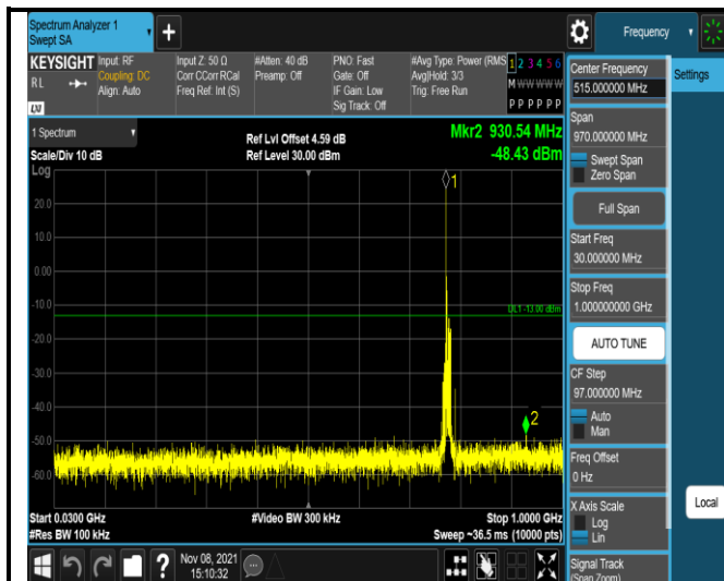
Band13-10MHz-QPSK-23230-1RB#0- Range1:30~1000MHz
