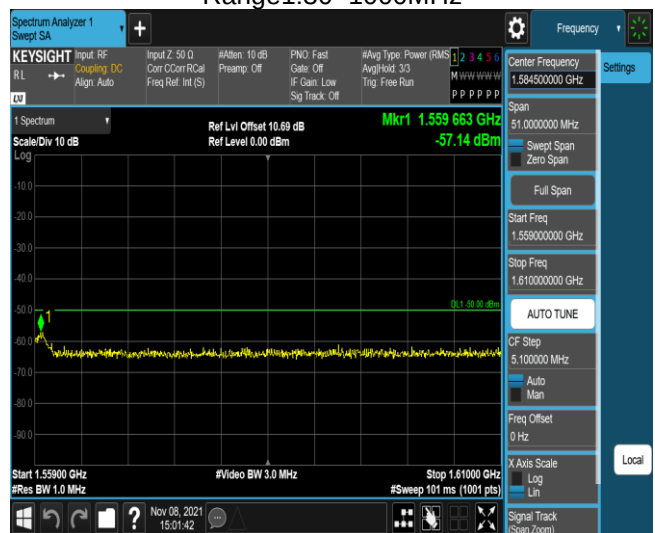
Band13-5MHz-QPSK-23230-1RB#0- Range3:1559~1610MHz
