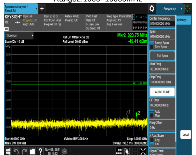
Band13-10MHz-16QAM-23230-1RB#0- Range1:30~1000MHz
