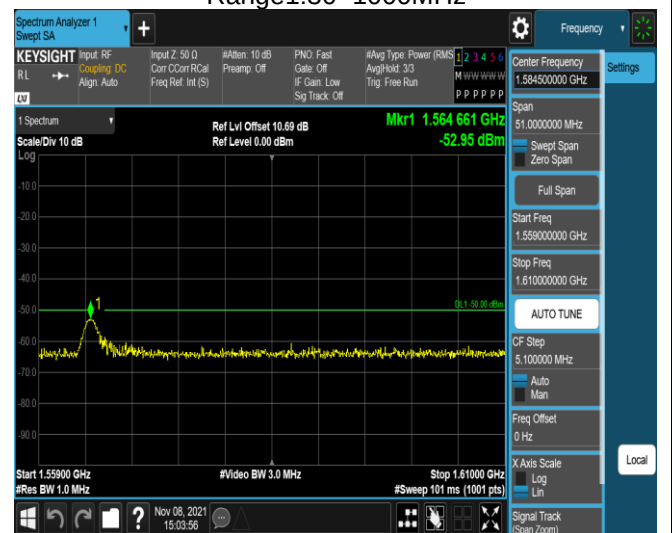
Band13-5MHz-16QAM-23255-1RB#0- Range3:1559~1610MHz
