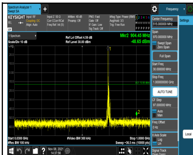
Band12-10MHz-16QAM-23060-1RB#0- Range1:30~1000MHz
