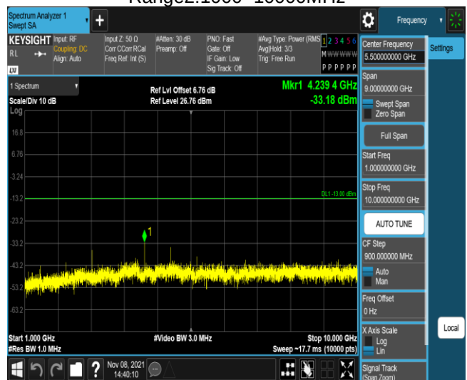
Band12-10MHz-16QAM-23130-1RB#0- Range2:1000~10000MHz
