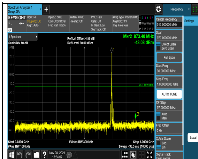
Band17-5MHz-QPSK-23755-1RB#0- Range1:30~1000MHz
