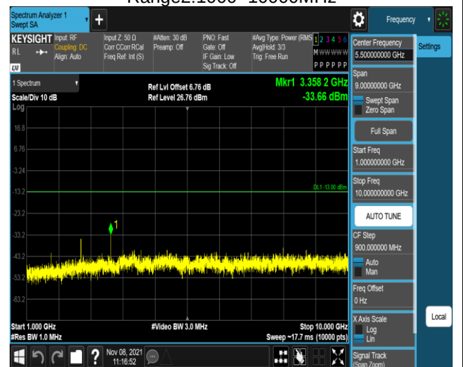
Band5-10MHz-16QAM-20600-1RB#0- Range2:1000~10000MHz
