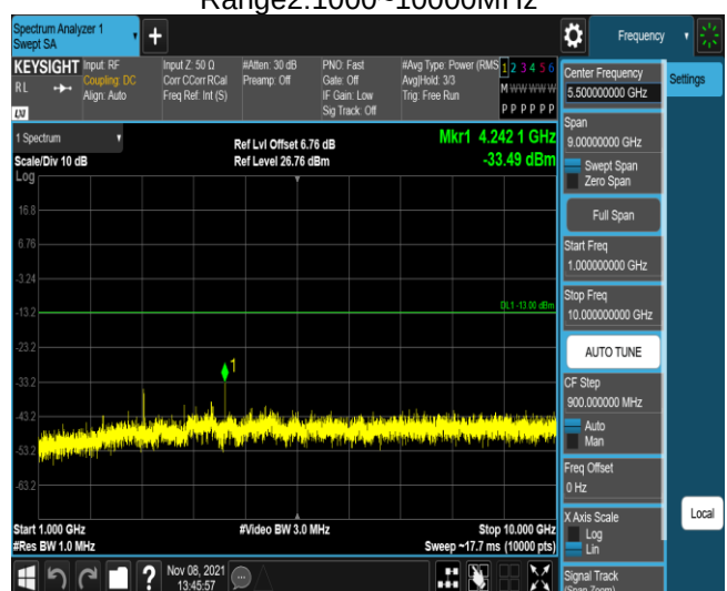
Band12-1.4MHz-16QAM-23095-1RB#0- Range2:1000~10000MHz
