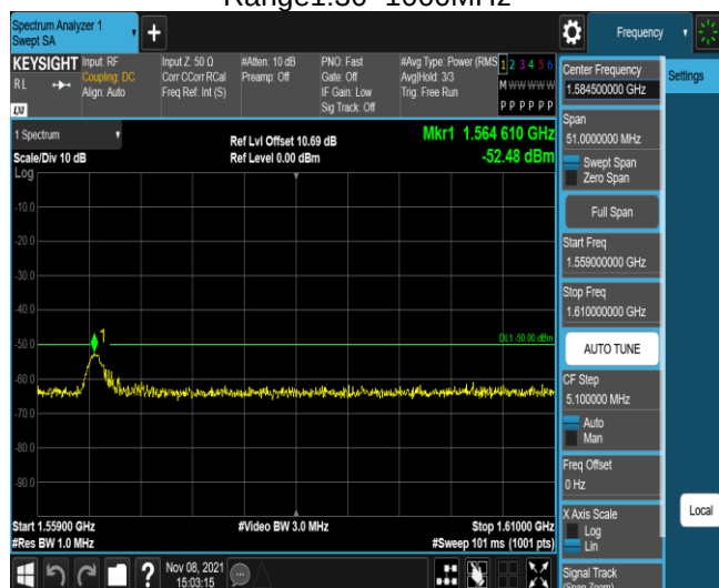
Band13-5MHz-QPSK-23255-1RB#0- Range3:1559~1610MHz
