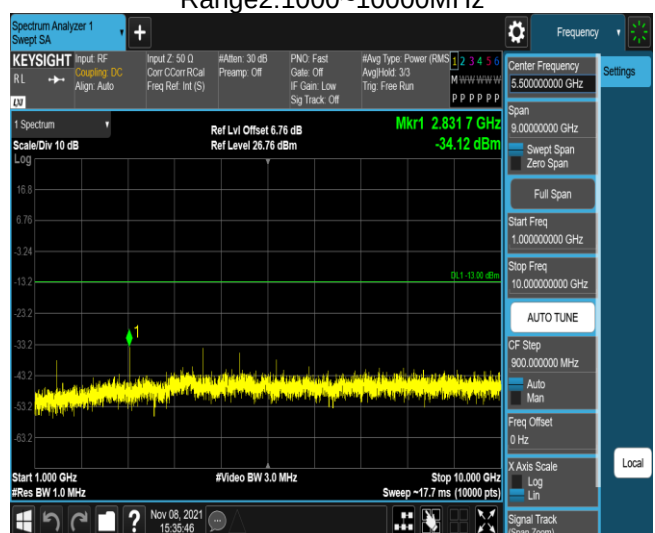
Band17-5MHz-QPSK-23790-1RB#0- Range2:1000~10000MHz
