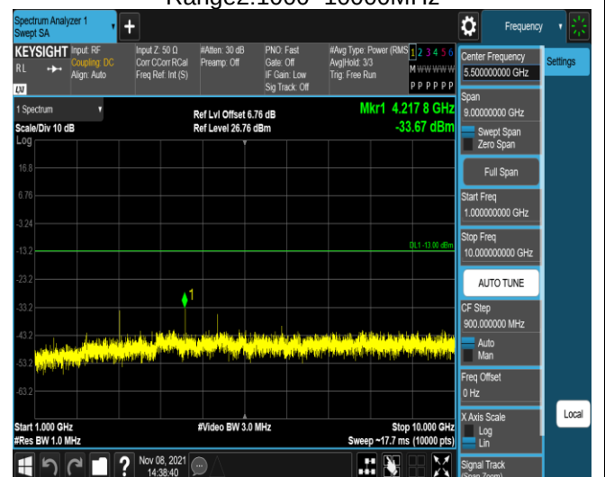
Band12-10MHz-QPSK-23095-1RB#0- Range2:1000~10000MHz
