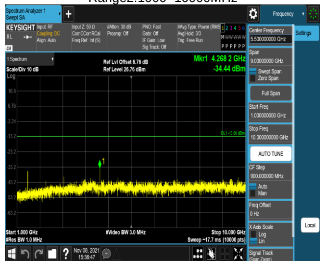
Band17-5MHz-QPSK-23825-1RB#0- Range2:1000~10000MHz
