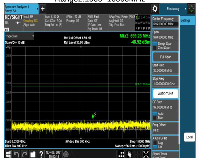
Band13-5MHz-16QAM-23205-1RB#0- Range1:30~1000MHz
