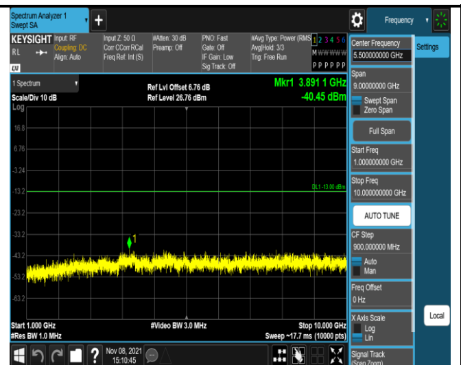
Band13-10MHz-QPSK-23230-1RB#0- Range2:1000~10000MHz
