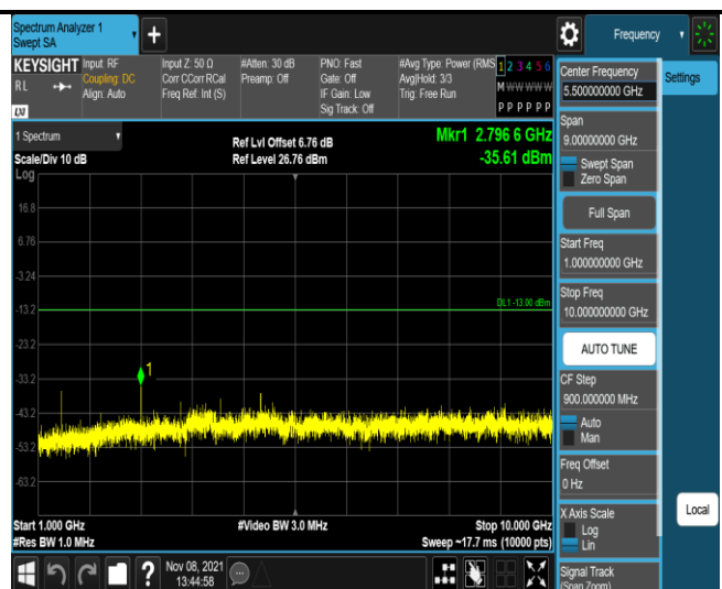
Band12-1.4MHz-16QAM-23017-1RB#0- Range2:1000~10000MHz
