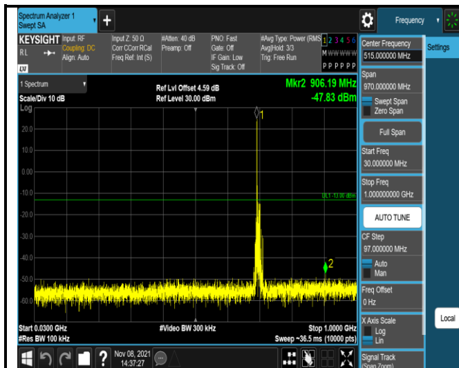
Band12-10MHz-QPSK-23060-1RB#0- Range1:30~1000MHz
