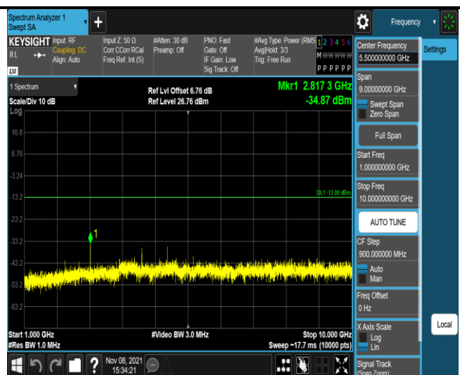
Band17-5MHz-QPSK-23755-1RB#0- Range2:1000~10000MHz
