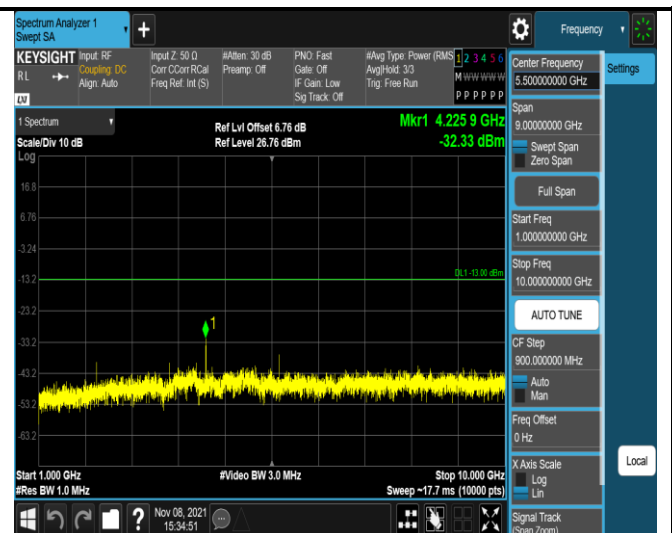
Band17-5MHz-16QAM-23755-1RB#0- Range2:1000~10000MHz
