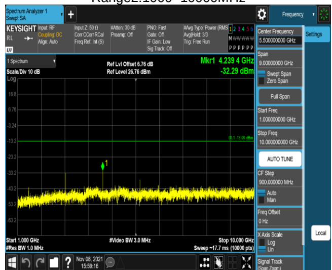
Band17-10MHz-QPSK-23800-1RB#0- Range2:1000~10000MHz
