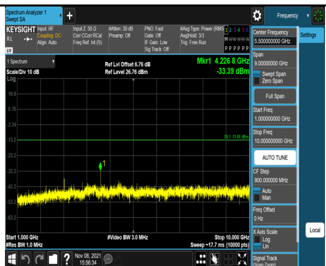
Band17-10MHz-QPSK-23780-1RB#0- Range2:1000~10000MHz
