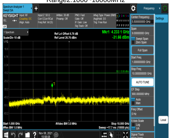
Band17-10MHz-QPSK-23790-1RB#0- Range2:1000~10000MHz
