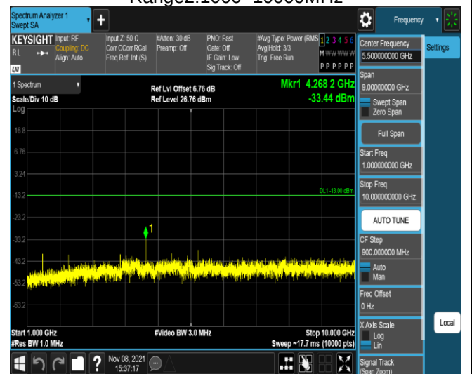
Band17-5MHz-16QAM-23825-1RB#0- Range2:1000~10000MHz
