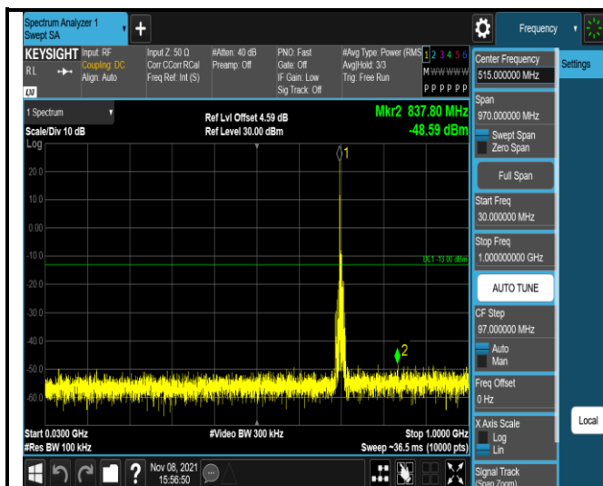
Band17-10MHz-16QAM-23780-1RB#0- Range1:30~1000MHz
