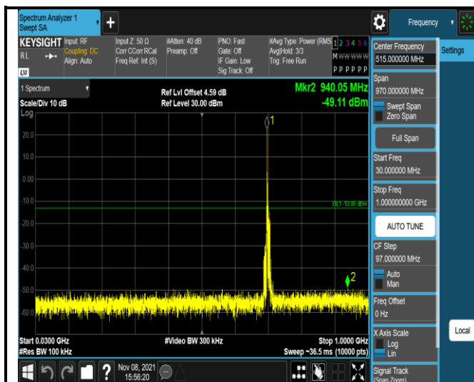
Band17-10MHz-QPSK-23780-1RB#0- Range1:30~1000MHz
