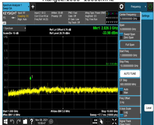
Band17-10MHz-16QAM-23800-1RB#0- Range2:1000~10000MHz
