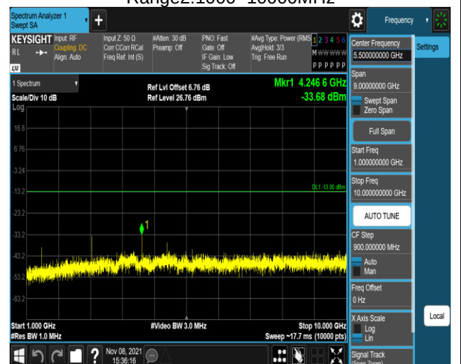
Band17-5MHz-16QAM-23790-1RB#0- Range2:1000~10000MHz
