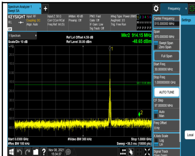
Band17-5MHz-16QAM-23755-1RB#0- Range1:30~1000MHz
