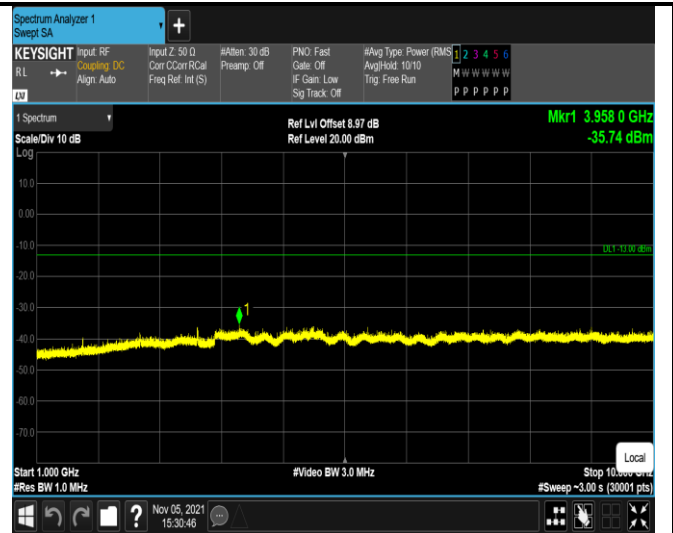
Band5-4183-1000~10000MHz
