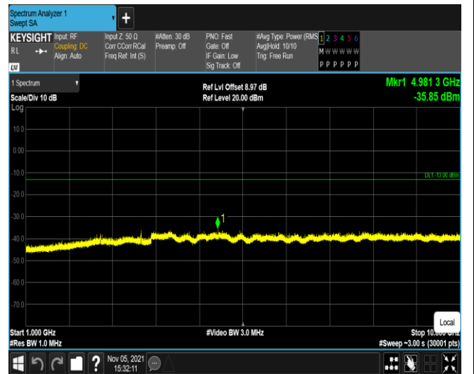
Band5-4233-1000~10000MHz
