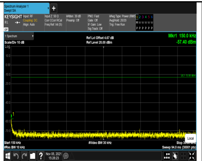
Band5-4132-0.15~30MHz
