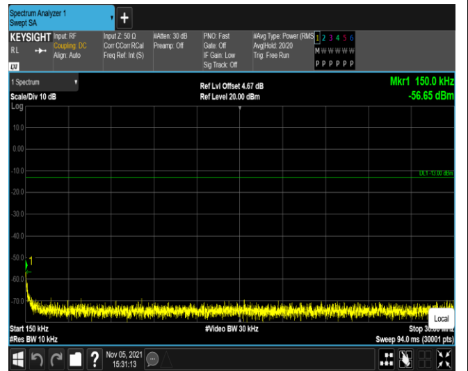
Band5-4233-0.15~30MHz
