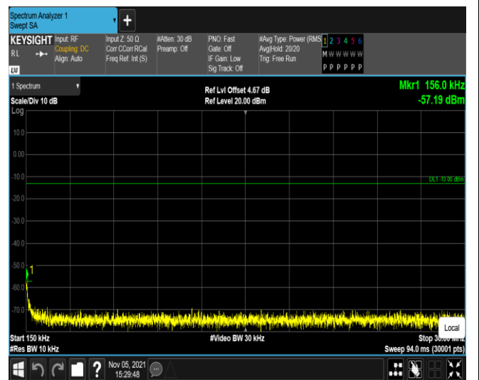
Band5-4183-0.15~30MHz
