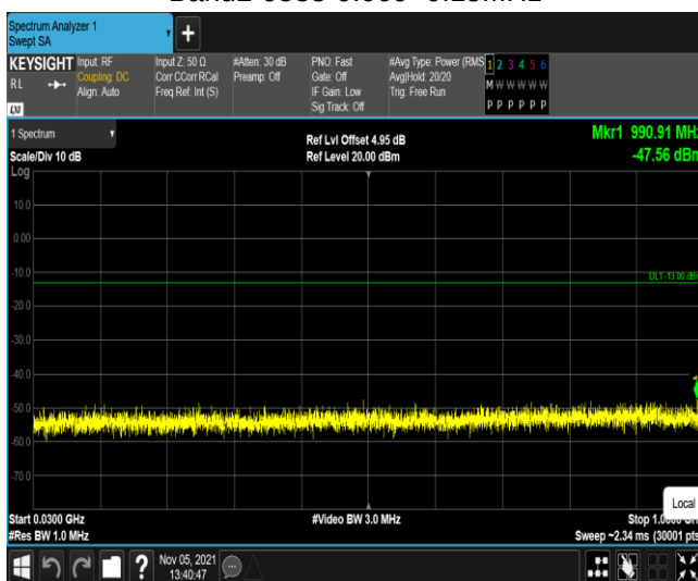
Band2-9538-30~1000MHz
