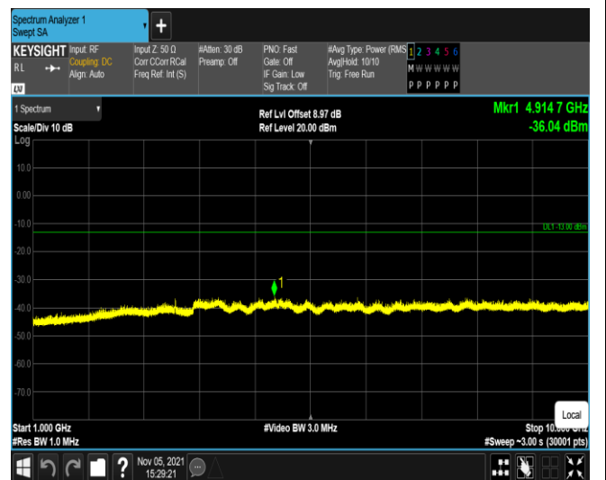
Band5-4132-1000~10000MHz
