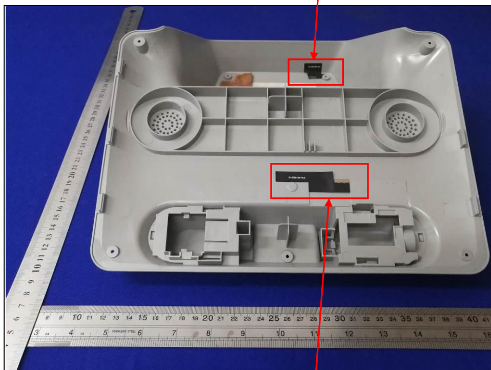
Diversity Antenna
