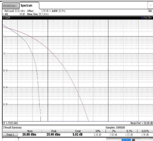
Band4-10MHz-QPSK-20175-50RB#0
