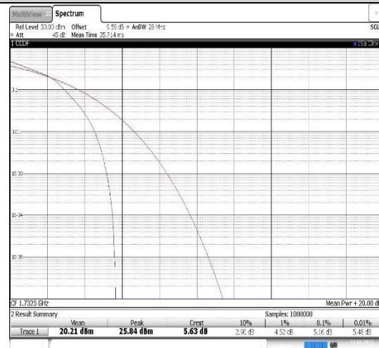
Band4-5MHz-16QAM-20175-25RB#0
