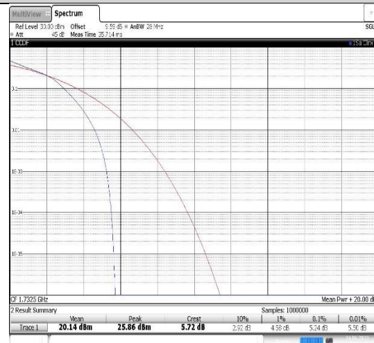
Band4-10MHz-16QAM-20175-50RB#0
