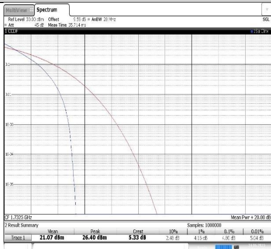
Band4-15MHz-QPSK-20175-75RB#0
