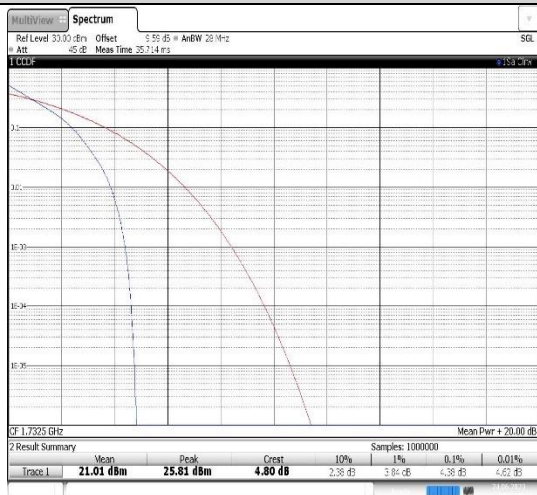
Band4-5MHz-QPSK-20175-25RB#0
