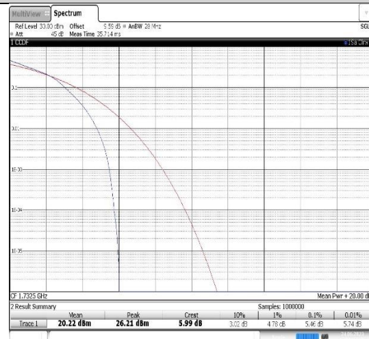
Band4-15MHz-16QAM-20175-75RB#0
