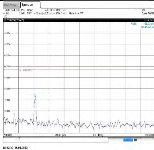
Band2-9400-5-0.009~0.15MHz
